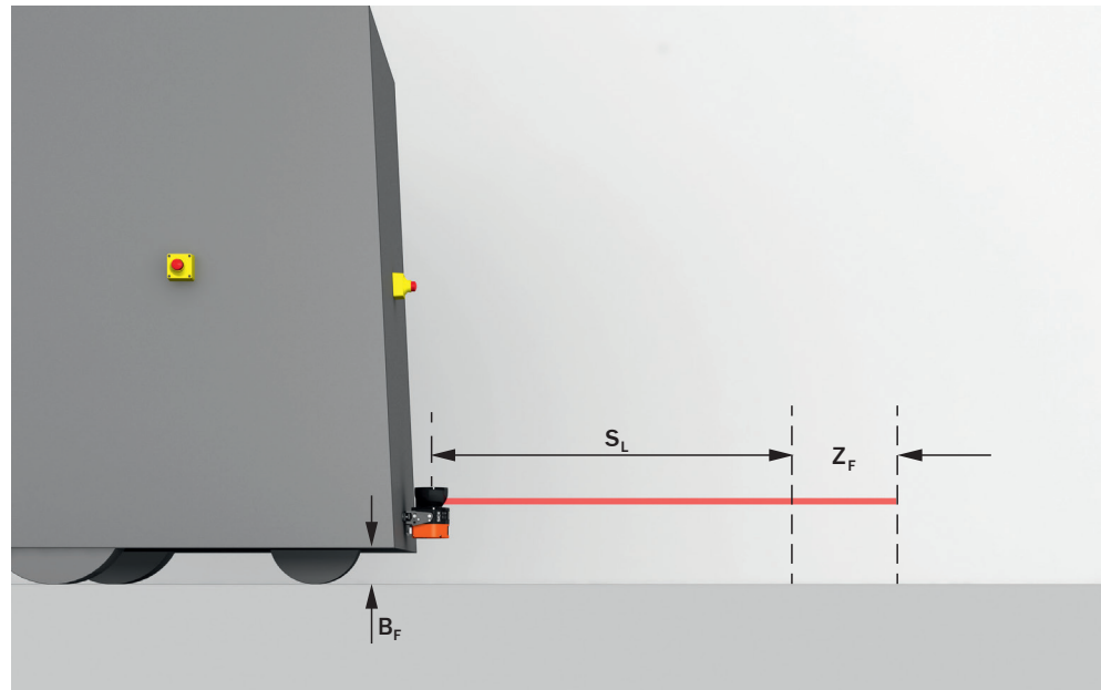
Figure 27: flat-rate supplement Z_F for lack of ground clearance
