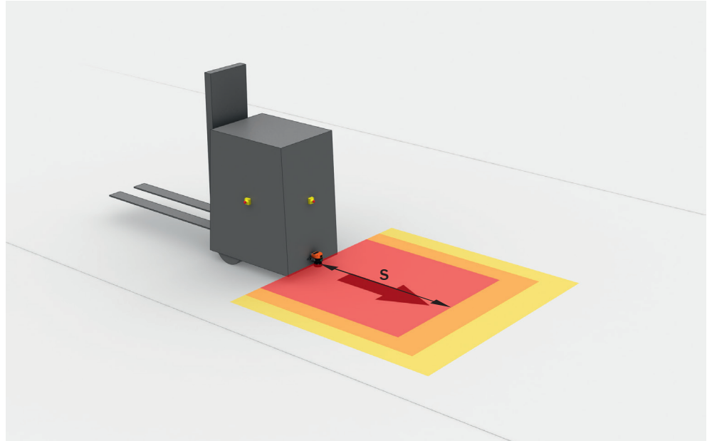
Figure 26: Mobile application in horizontal operation for hazardous area protection
