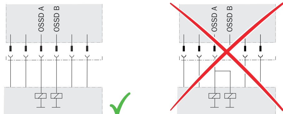
Figure 32: Dual-channel and separate connection of the OSSDs of an OSSD pair
