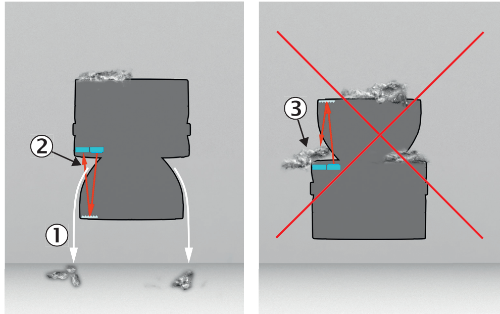
Figure 13: Device mounted with the optics cover facing downwards to prevent accumulation of contaminants on the contamination measurement feature
