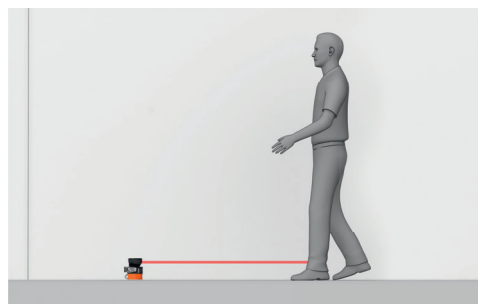
Figure 36: Prevent stepping over
