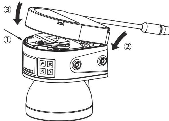
Figure 62: Installing the system plug on the safety laser scanner
