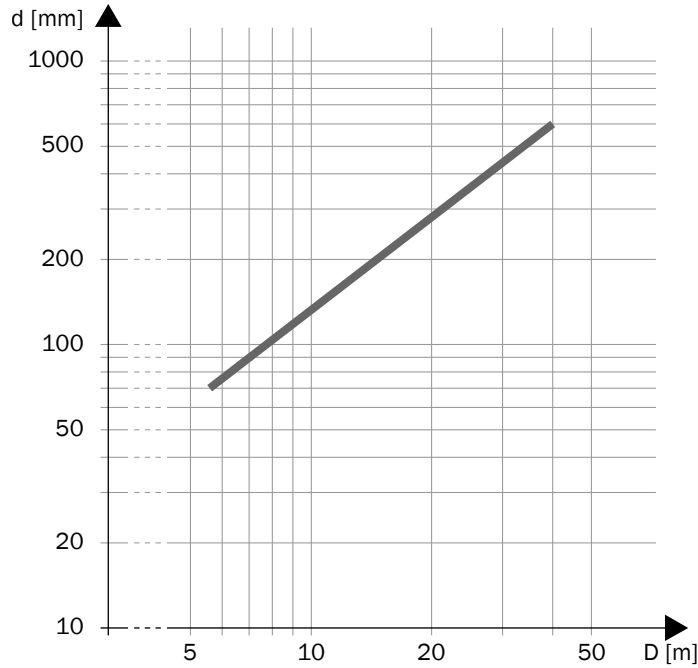
Figure 70: Scanning range and object size for warning fields
