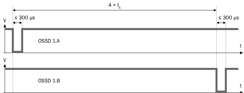
Figure 69: Duration and time offset for the switch-off tests in an OSSD pair
