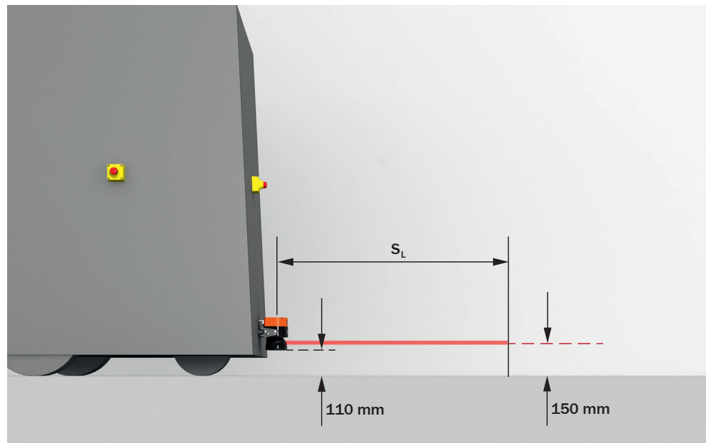
Figure 31: Recommended fitting height for inverted mounting 2)
