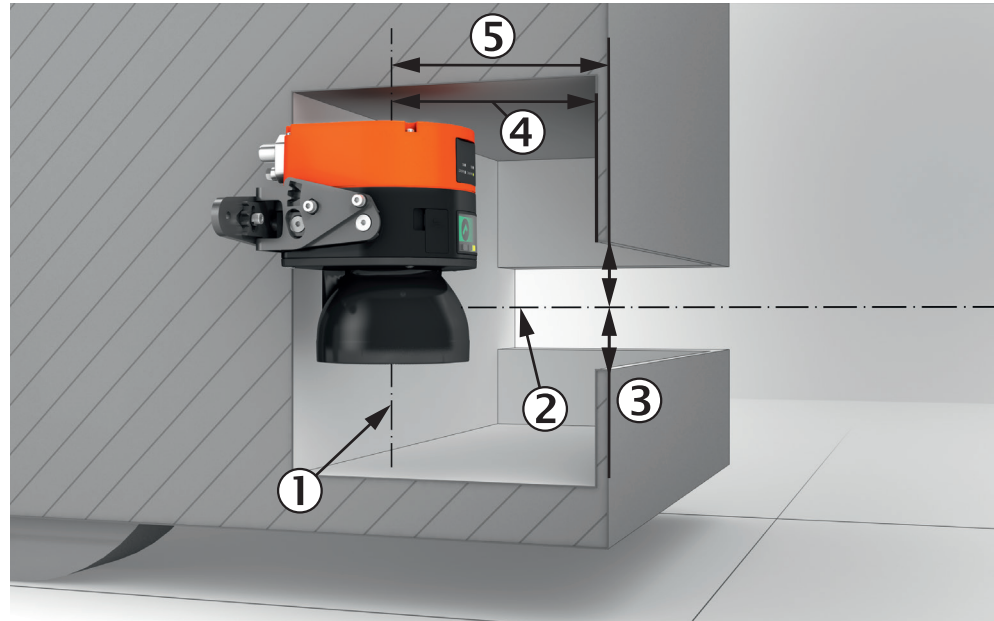
Figure 19: Mounting in vehicle paneling (example)
