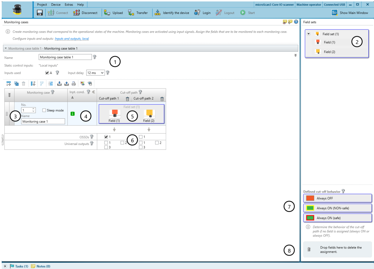
Figure 54: Monitoring cases
