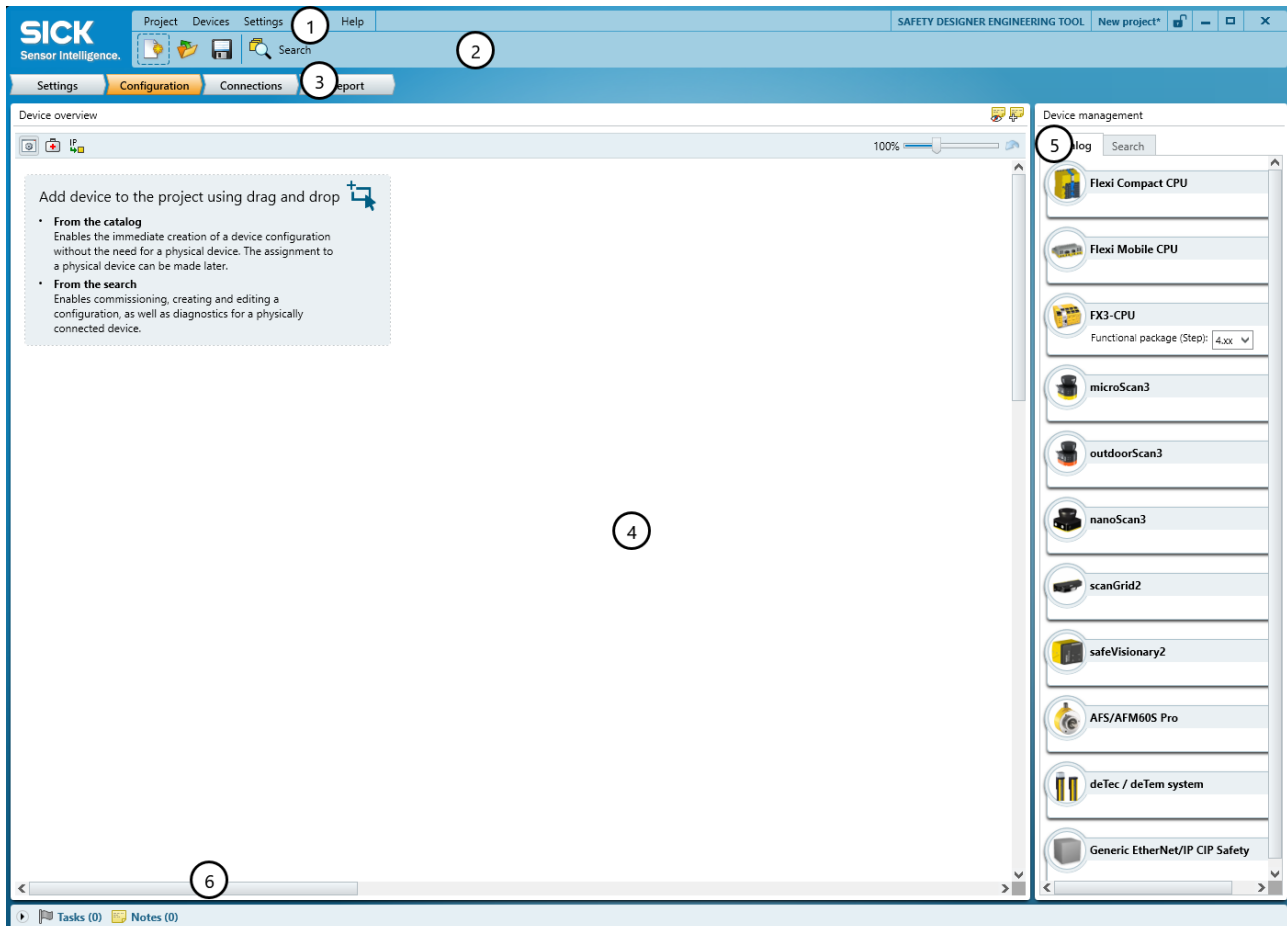
Figure 41: Software controls
