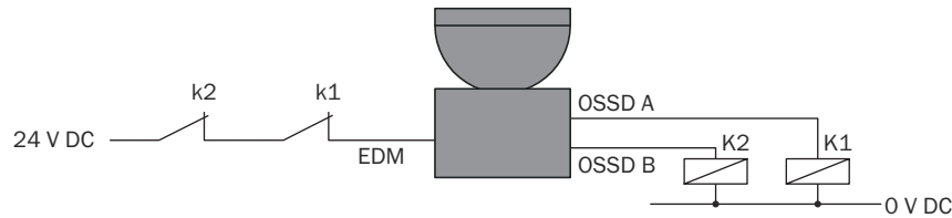
Figure 34: Electrical diagram of external device monitoring (EDM)
