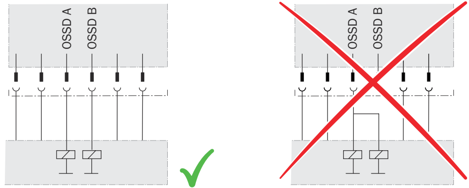
Figure 38: Connection of the OSSDs of an OSSD pair
