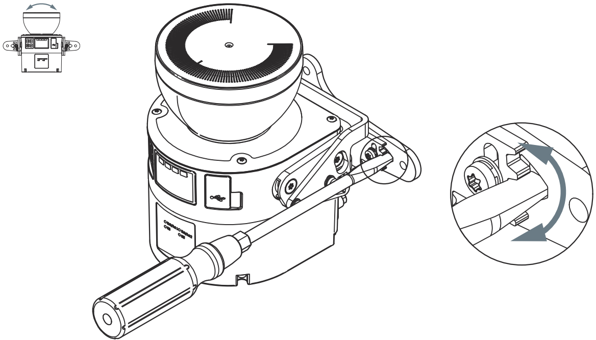
Figure 58: Alignment about the depth axis
