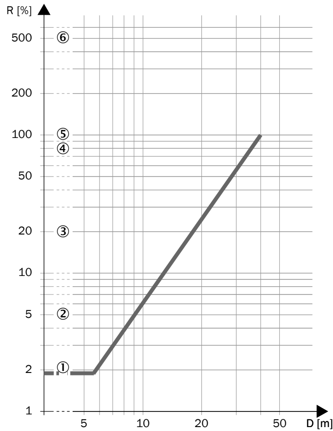
Figure 71: Scanning range and required remission for warning fields
