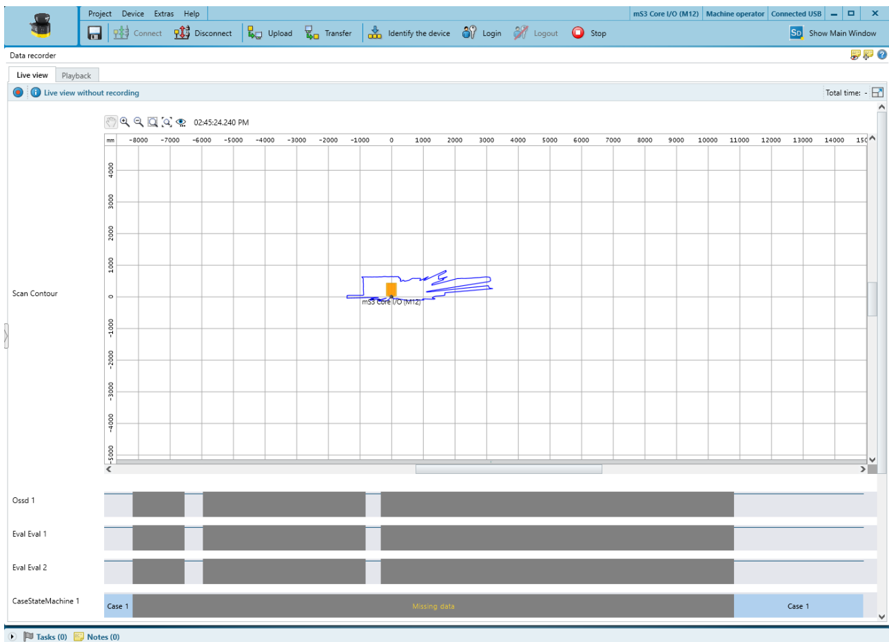
Figure 65: Data recorder
