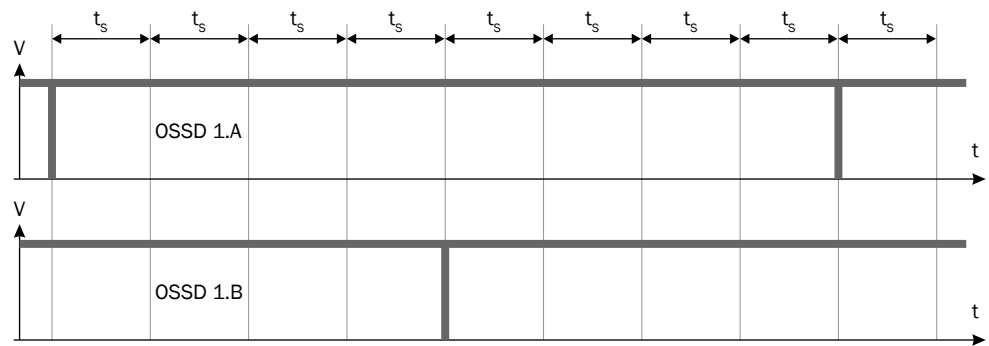
Figure 68: Switch-off tests
