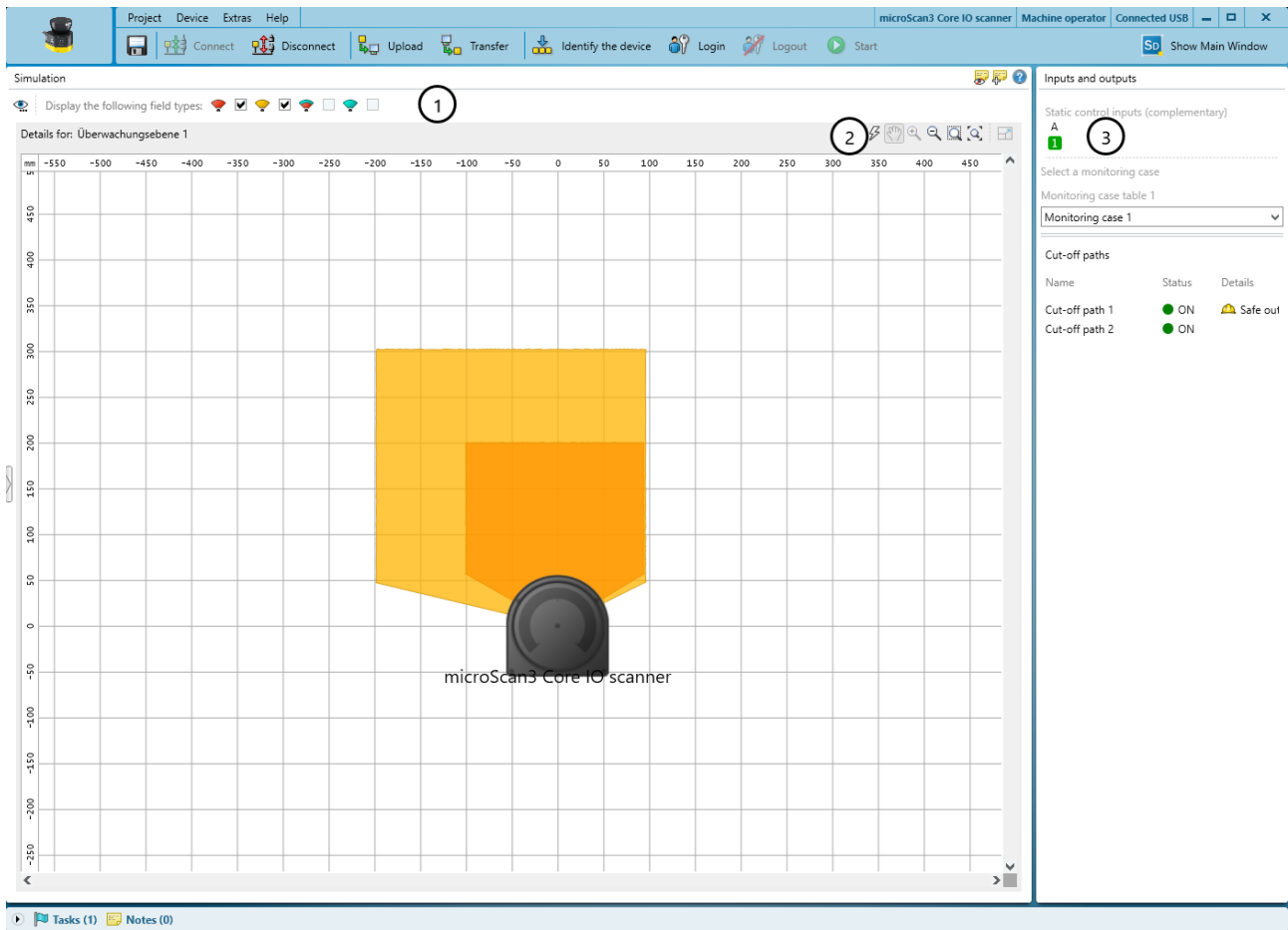
Figure 55: Simulation
