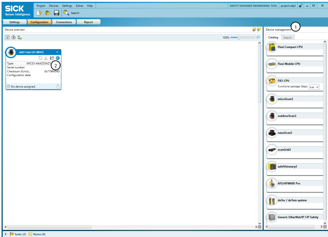
Figure 42: Configuration
