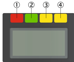
Figure 59: Status LEDs
