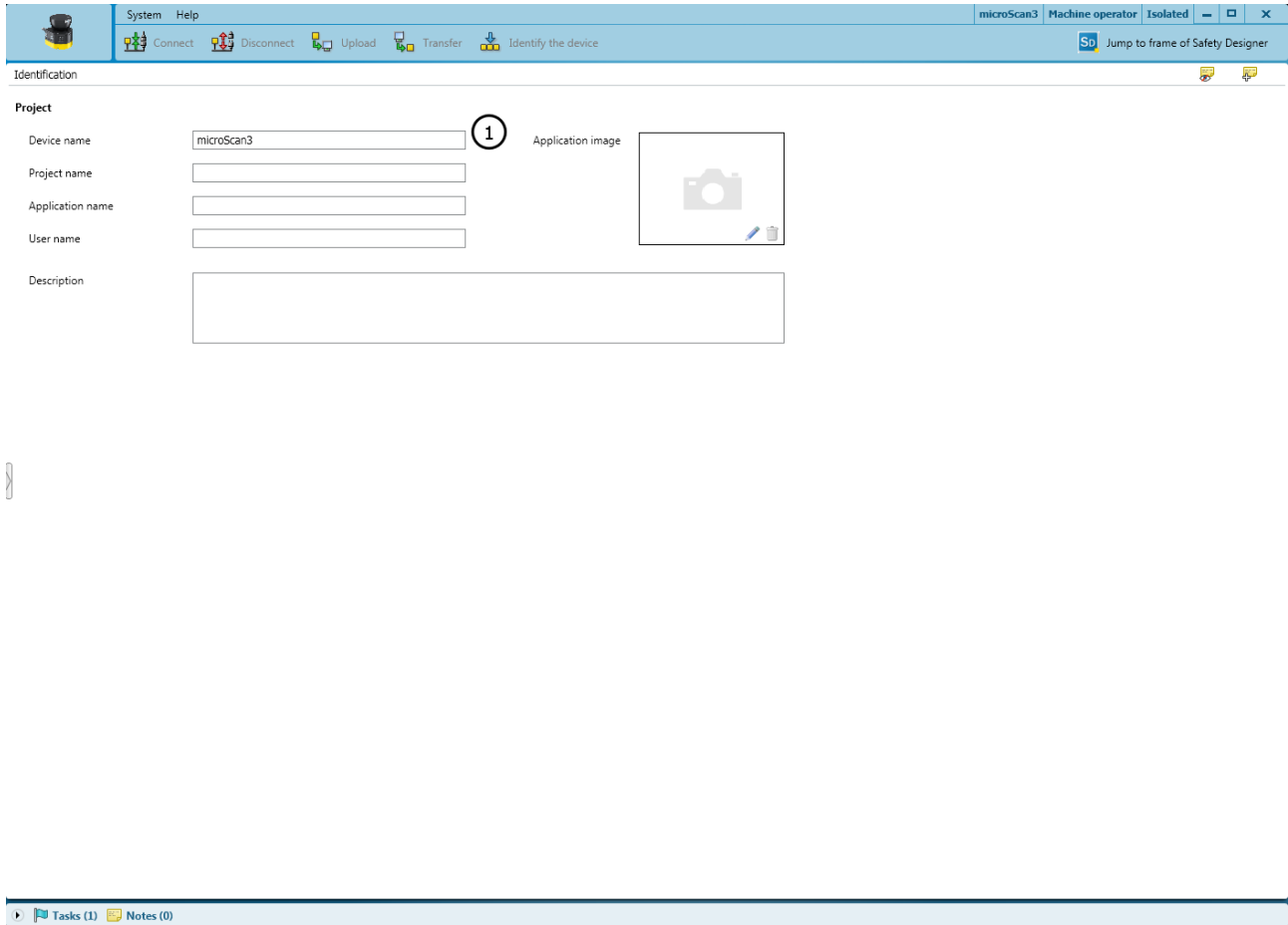
Figure 45: Identification
