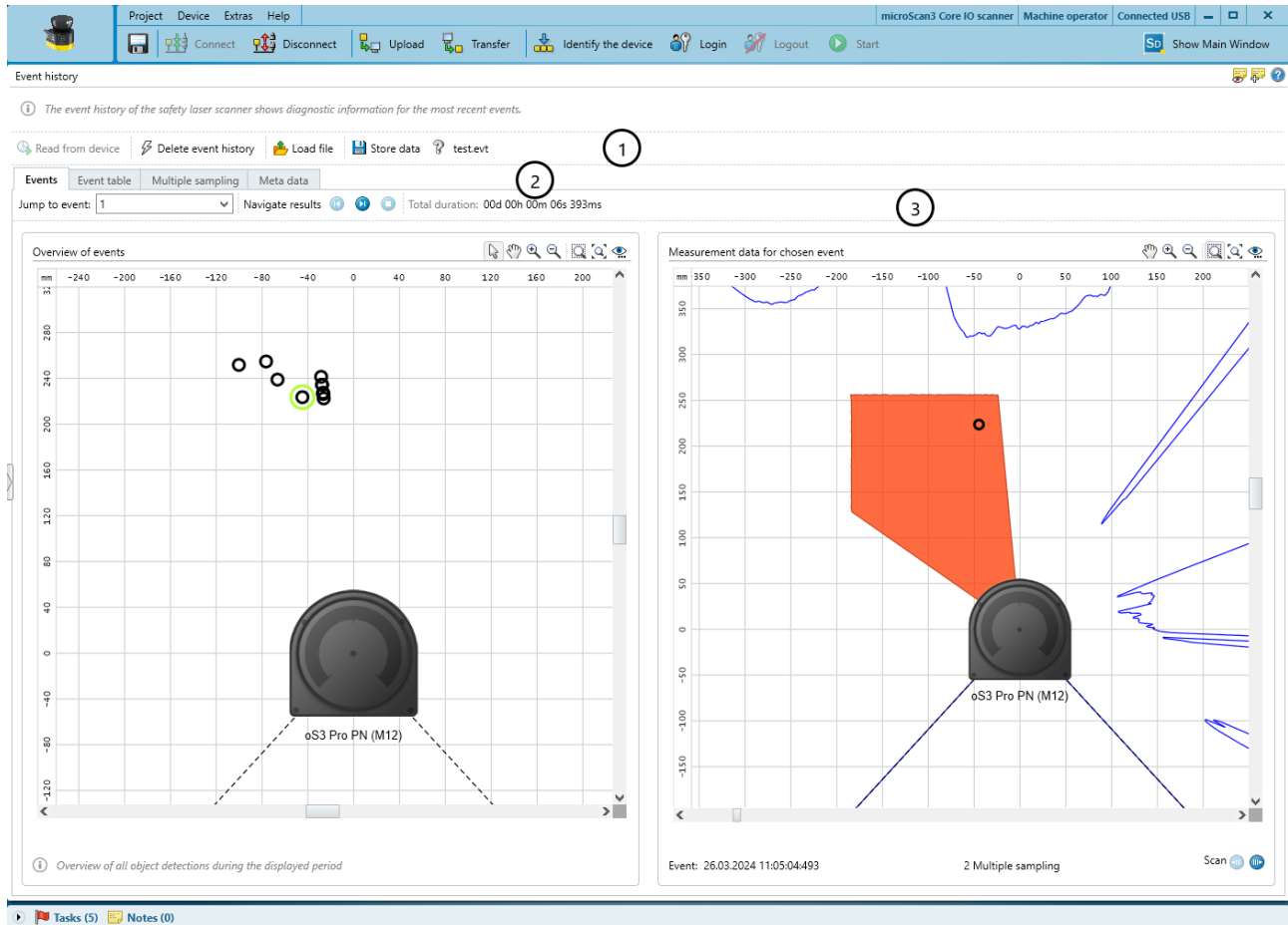
Figure 66: Event history
