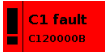
Figure 64: Error display
