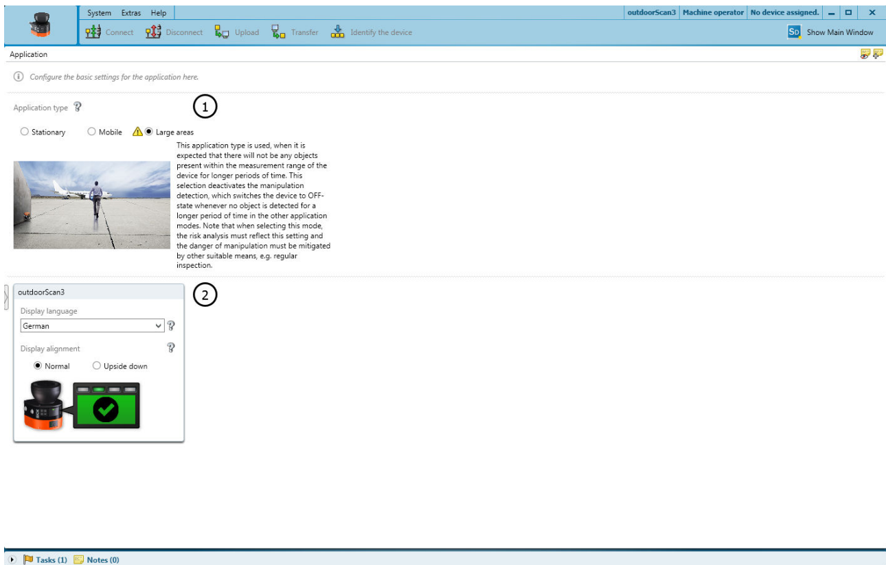
Figure 46: Application
