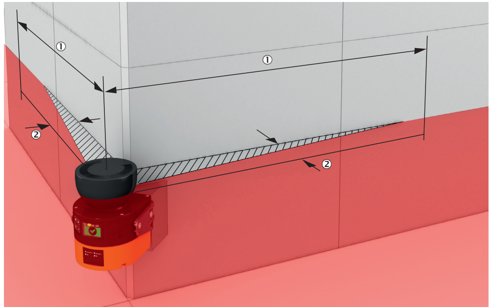
Figure 16: Unsecured areas
