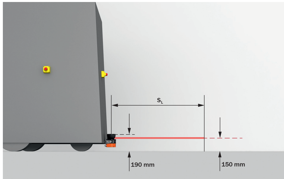
Figure 30: Recommended fitting height
