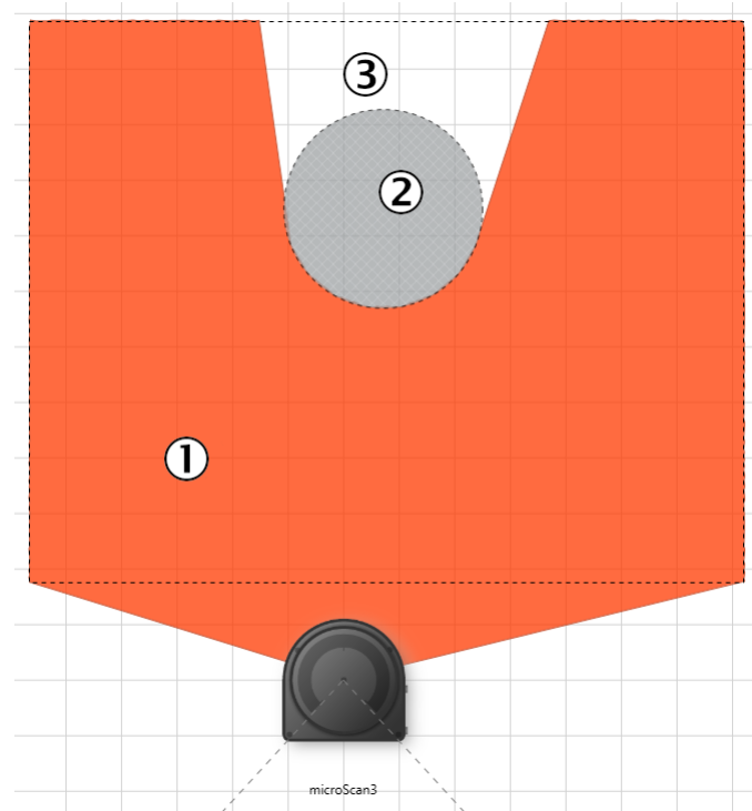
Figure 49: Area that cannot be monitored
