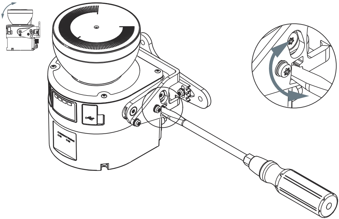
Figure 57: Alignment about the transverse axis
