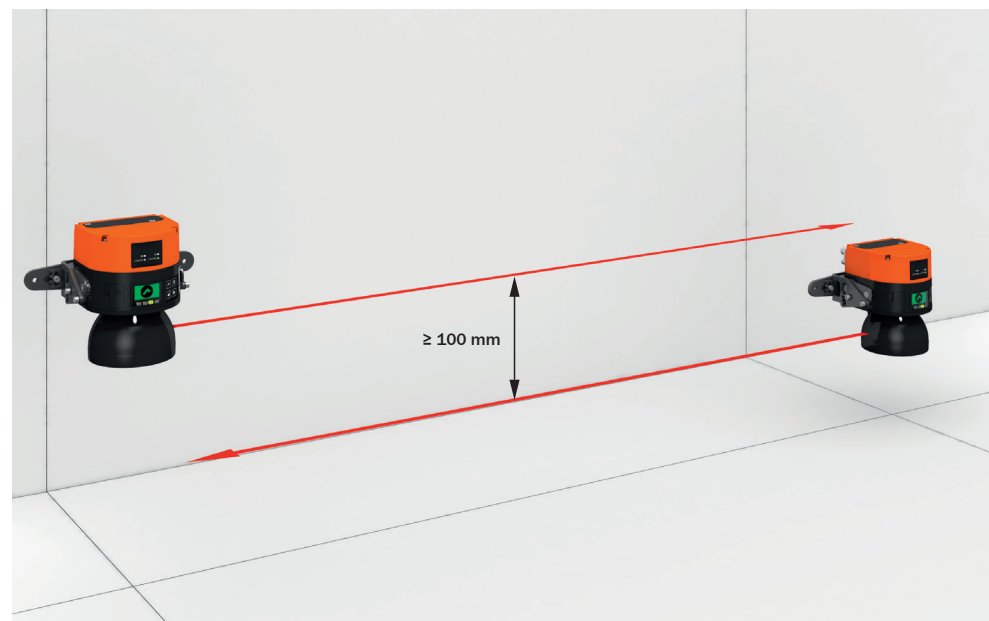
Figure 73: Mounting 2 safety laser scanners with the optics cover facing downward
