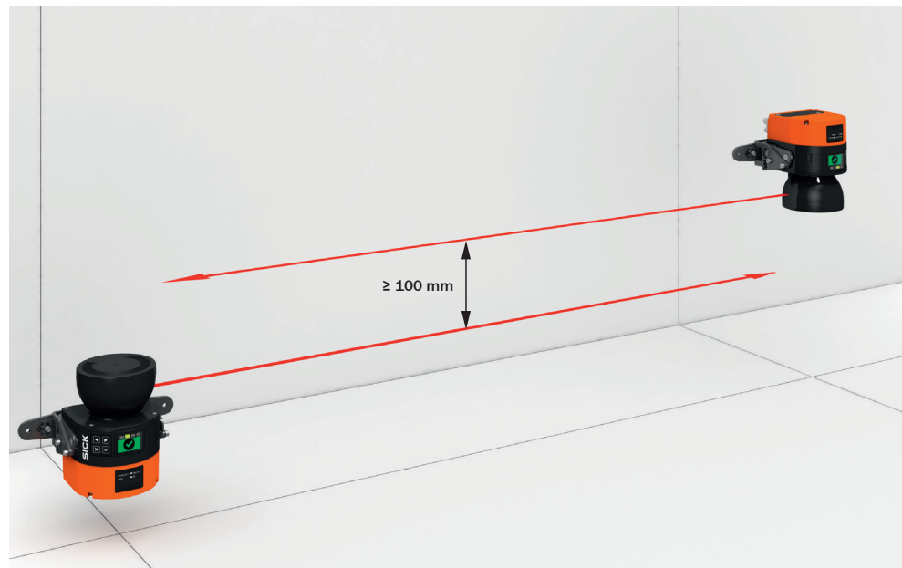
Figure 75: Mounting the upper safety laser scanner with the optics cover facing downward and mounting the lower safety laser scanner with the optics cover facing upward
