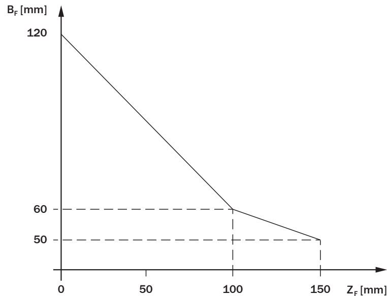
Figure 28: Minimum supplement for lack of ground clearance
