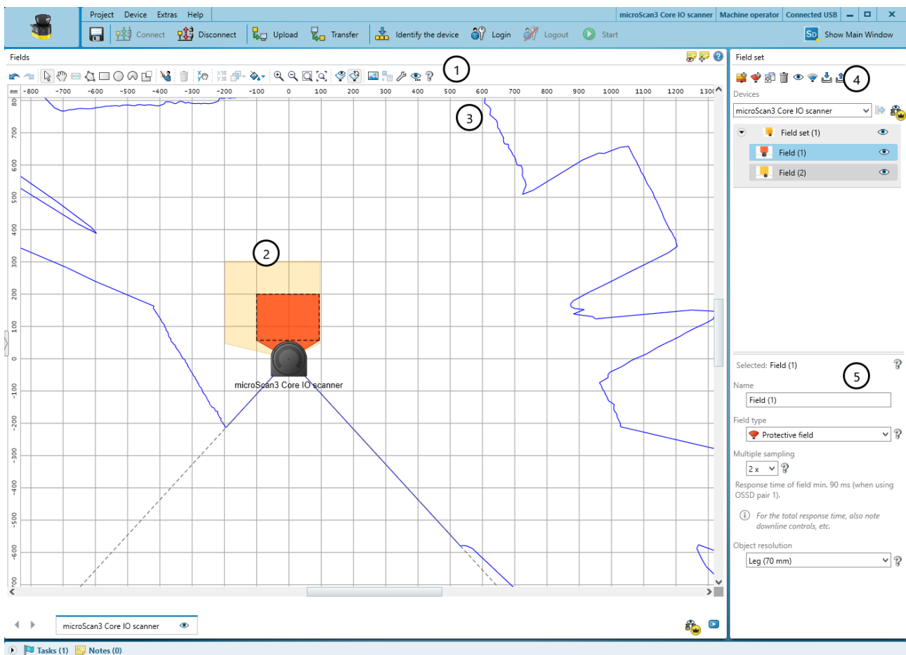
Figure 48: Field editor
