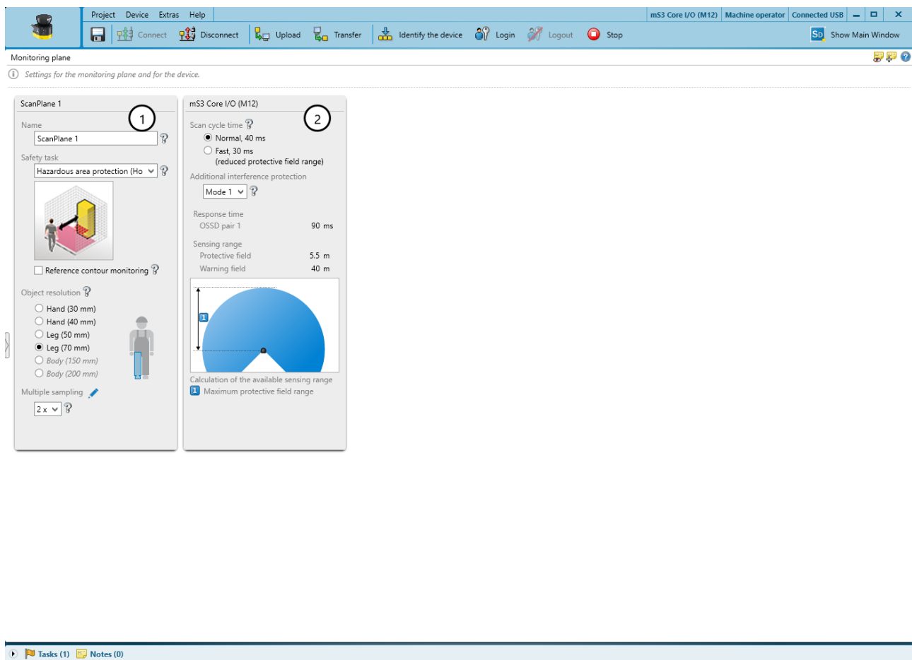
Figure 47: Monitoring plane
