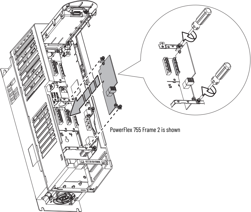
Figure 6 - Install Safety Option Module
