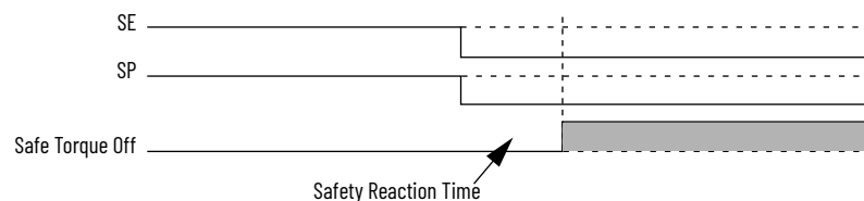
Figure 1 - Safety Reaction Timing Diagram
