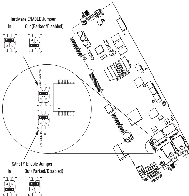
Figure 5 - PowerFlex 755TS Drives Jumper Locations
