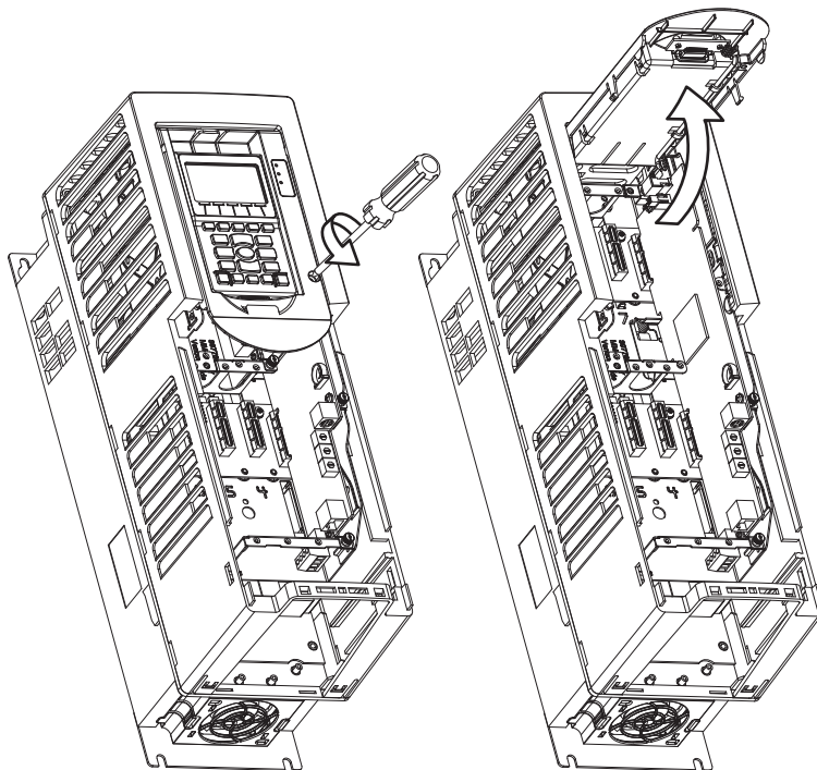
Panel-mounted Drives
