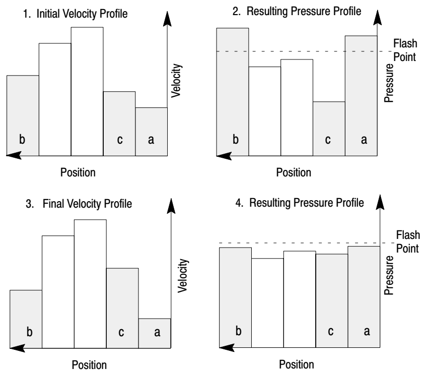
Figure 1.4 Flash Prevention Example
