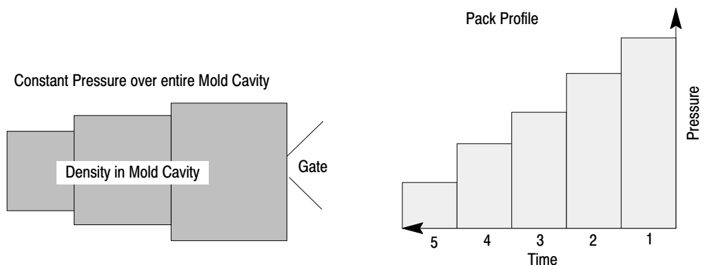
Figure 1.7 Even Cooling in Pack Phase
