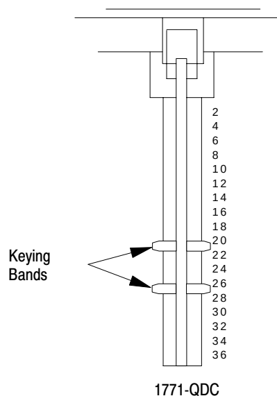
Figure 2.2 Keying Positions
