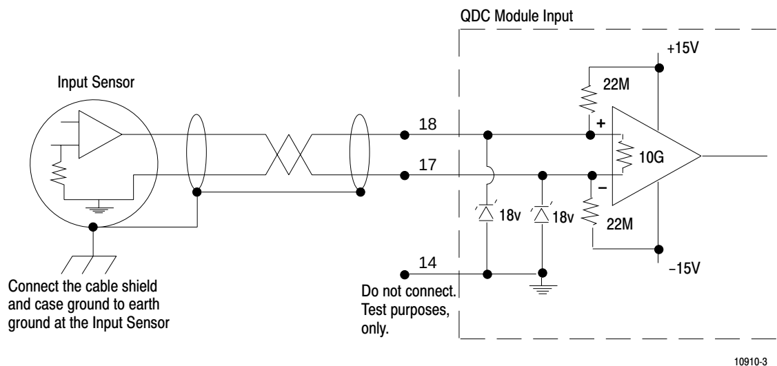
Figure 2.4 Shielding Differential Inputs
