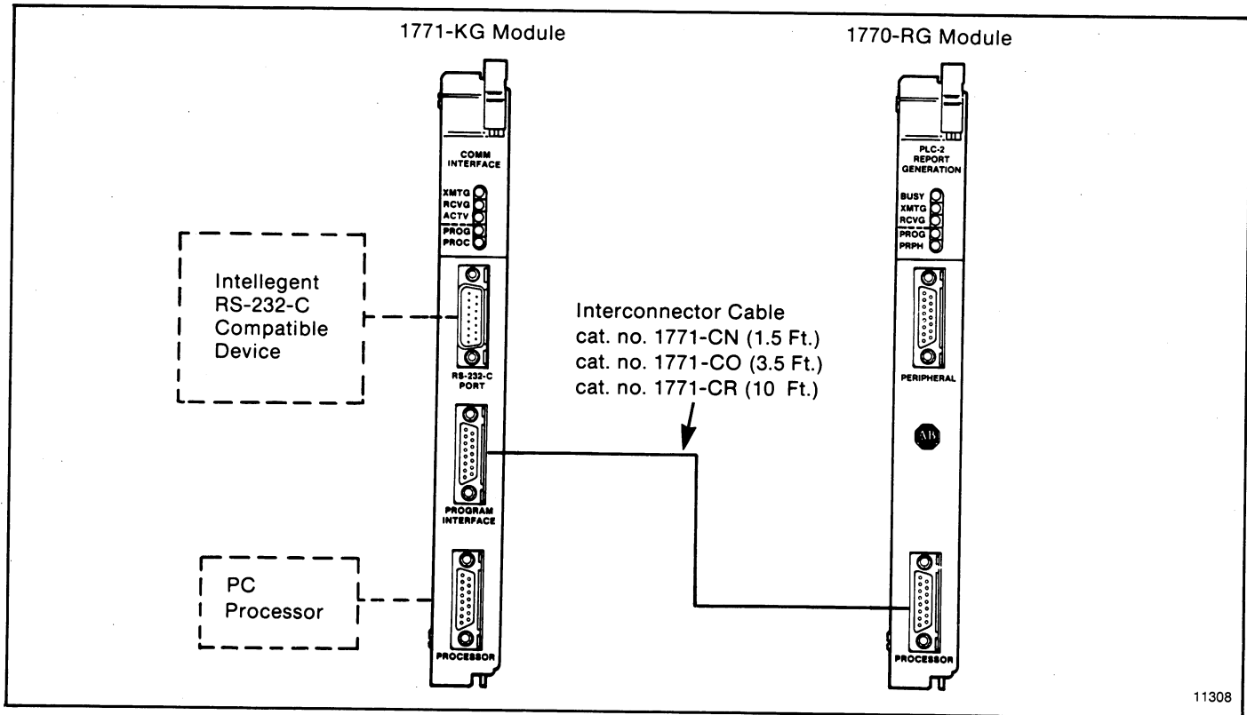
Figure 4.8 — Connection to a 1770-RG Module
