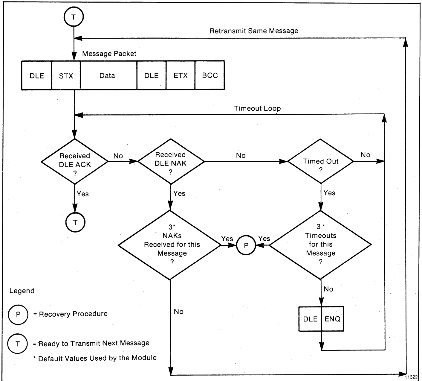
Figure 6.7 — Transmitter for Full-Duplex Protocol
