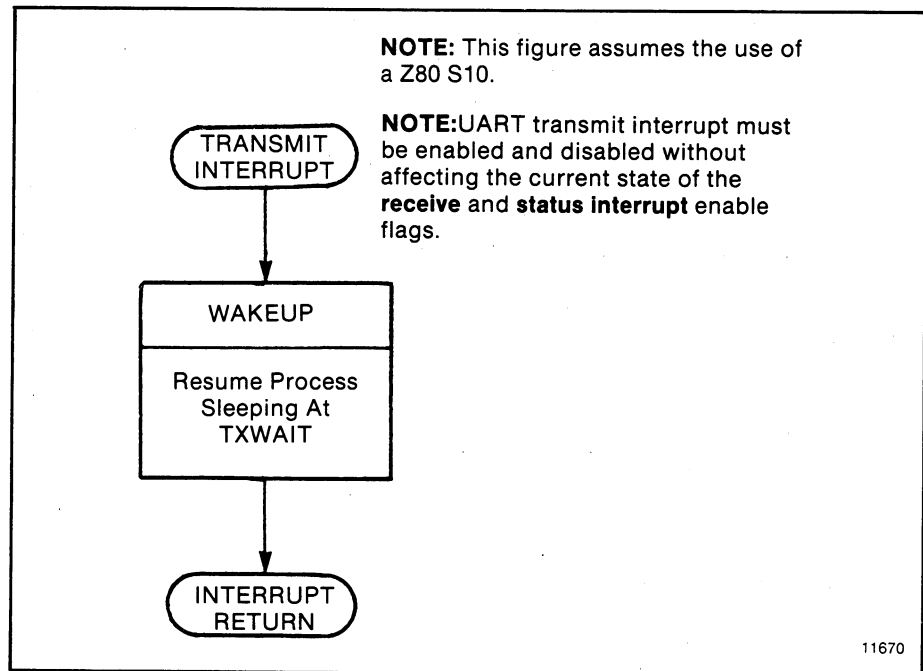
Figure D.18 — TRANSMIT INTERRUPT Subroutine
