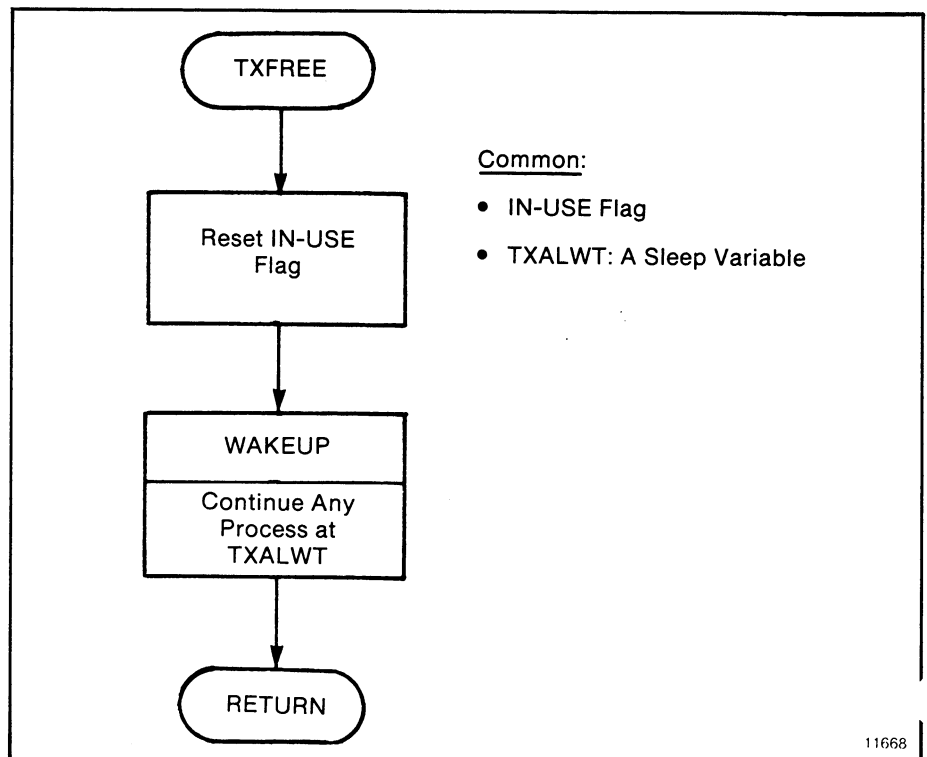
Figure D.16 — TXFREE Subroutine
