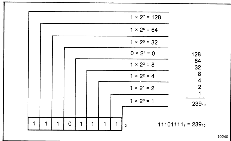
Figure C.1 — Binary Numbers
