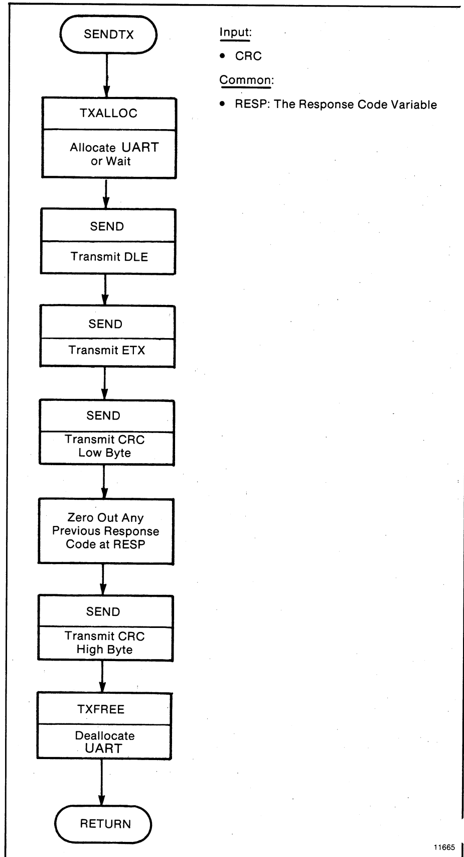
Figure D.13 — SENDTX Subroutine
