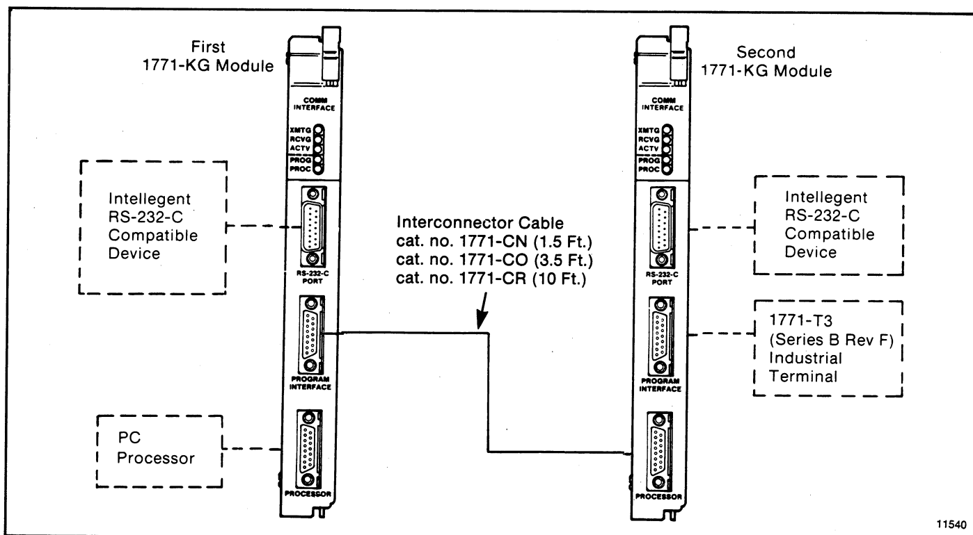
Figure 4.9 — Connection to a Second 1771-KG Module
