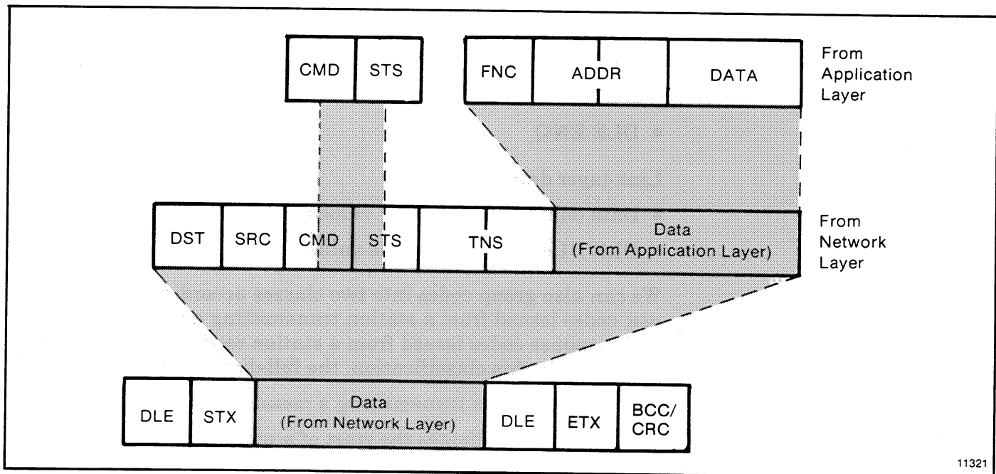
Figure 6.1 — Link Packet Format for Full-Duplex Protocol
