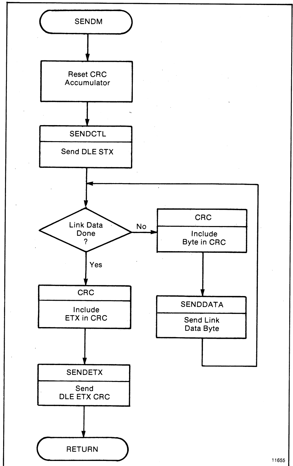
Figure D.4 — SENDM Subroutine
