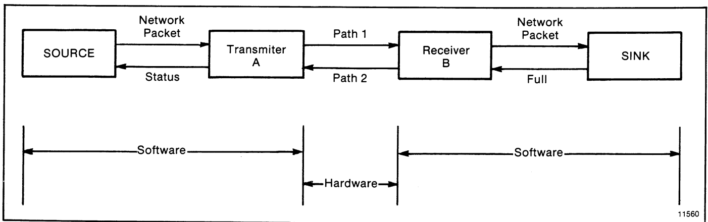
Figure 6.6 — Protocol Environment
