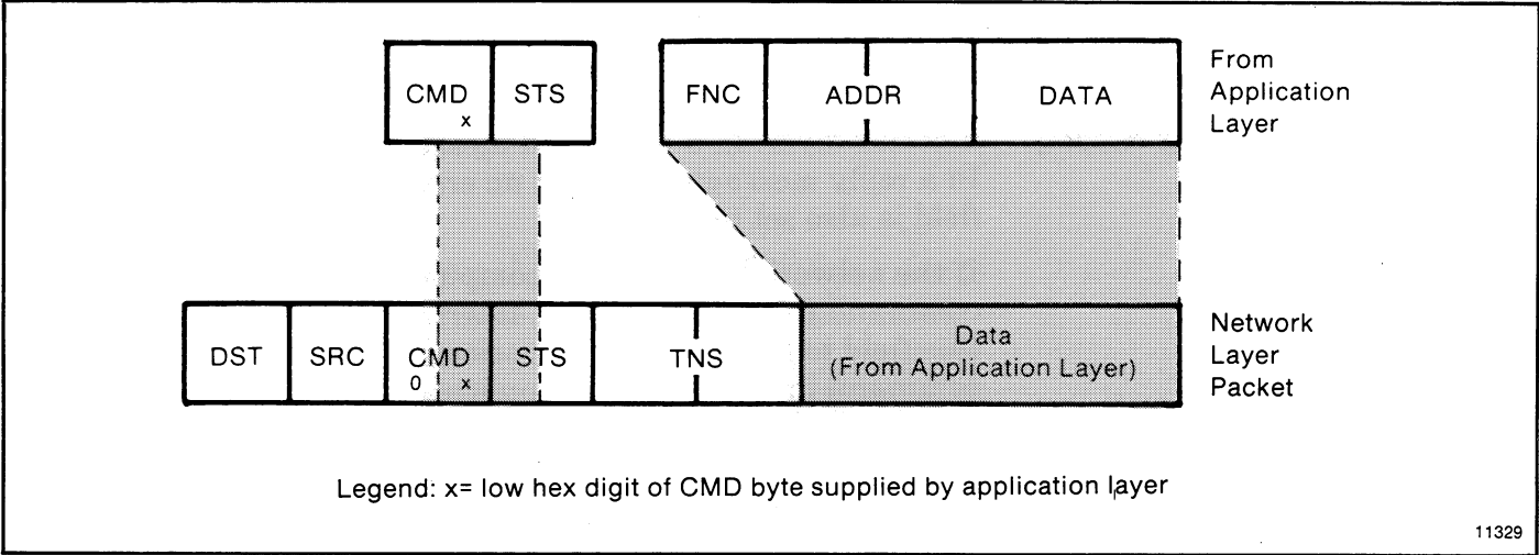
Figure 6.26 — Command Message Packet Format
