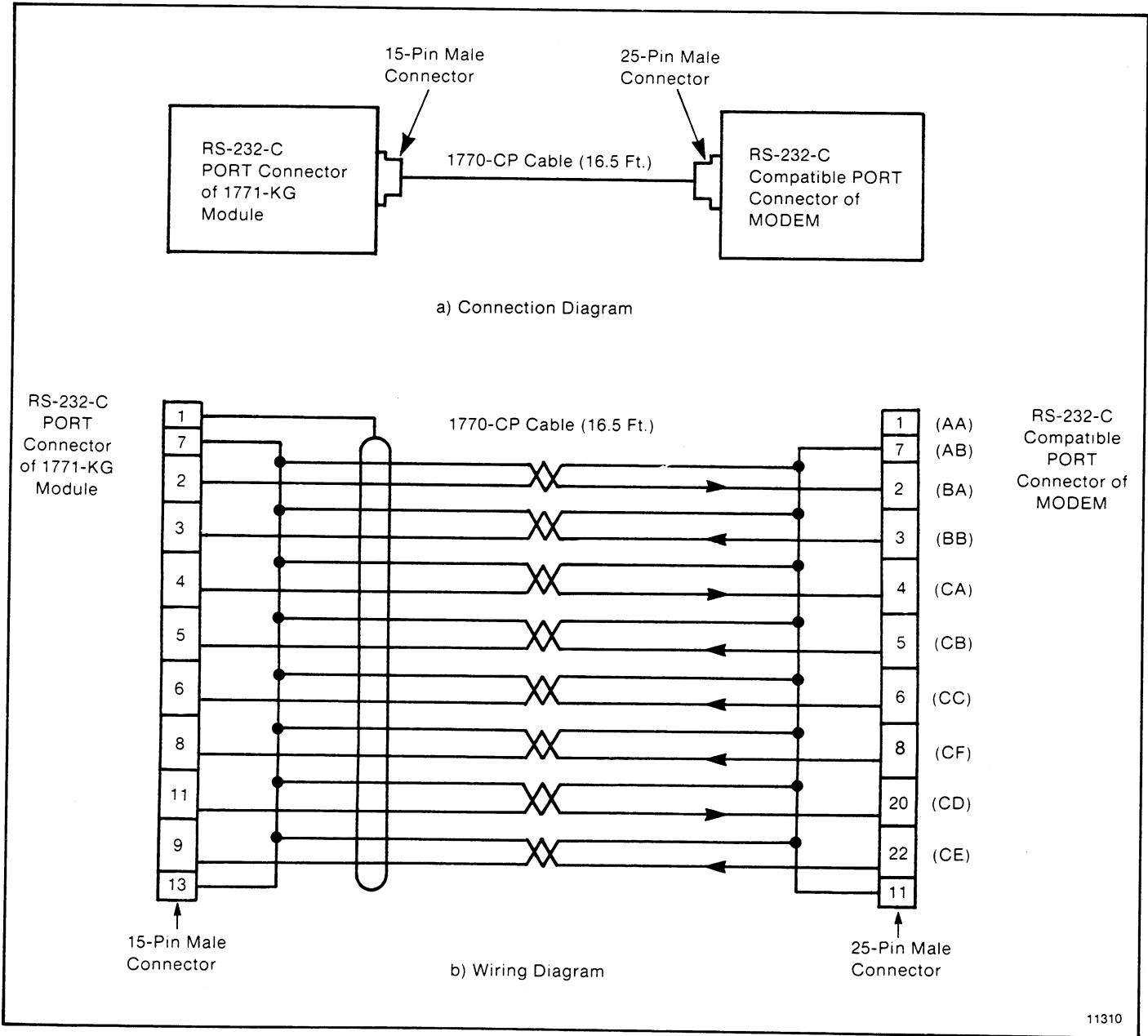
Figure 4.11 — Connection to a MODEM
