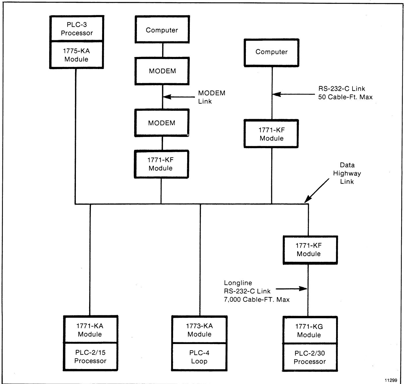
Figure 2.1 — Data Highway Network
