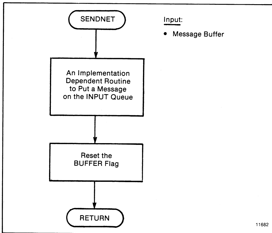
Figure D.30 — SENDNET Subroutine
