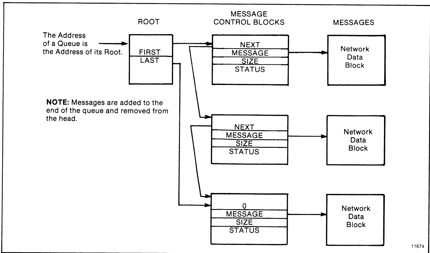
Figure D.22 — Message Queue
