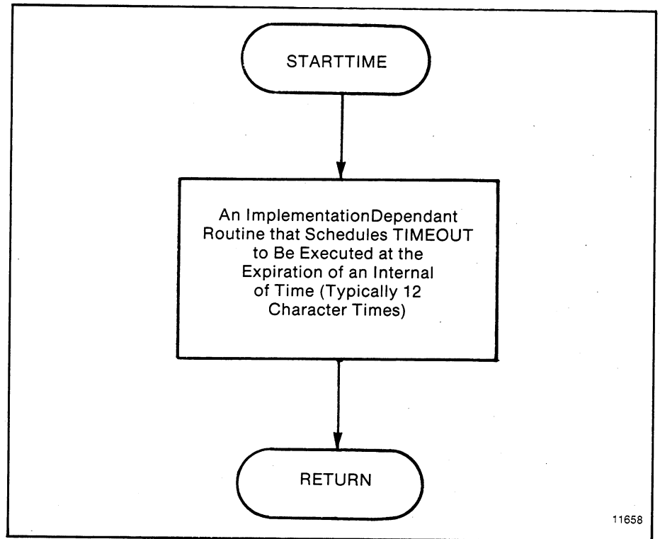
Figure D.6 — STARTTIME Subroutine
