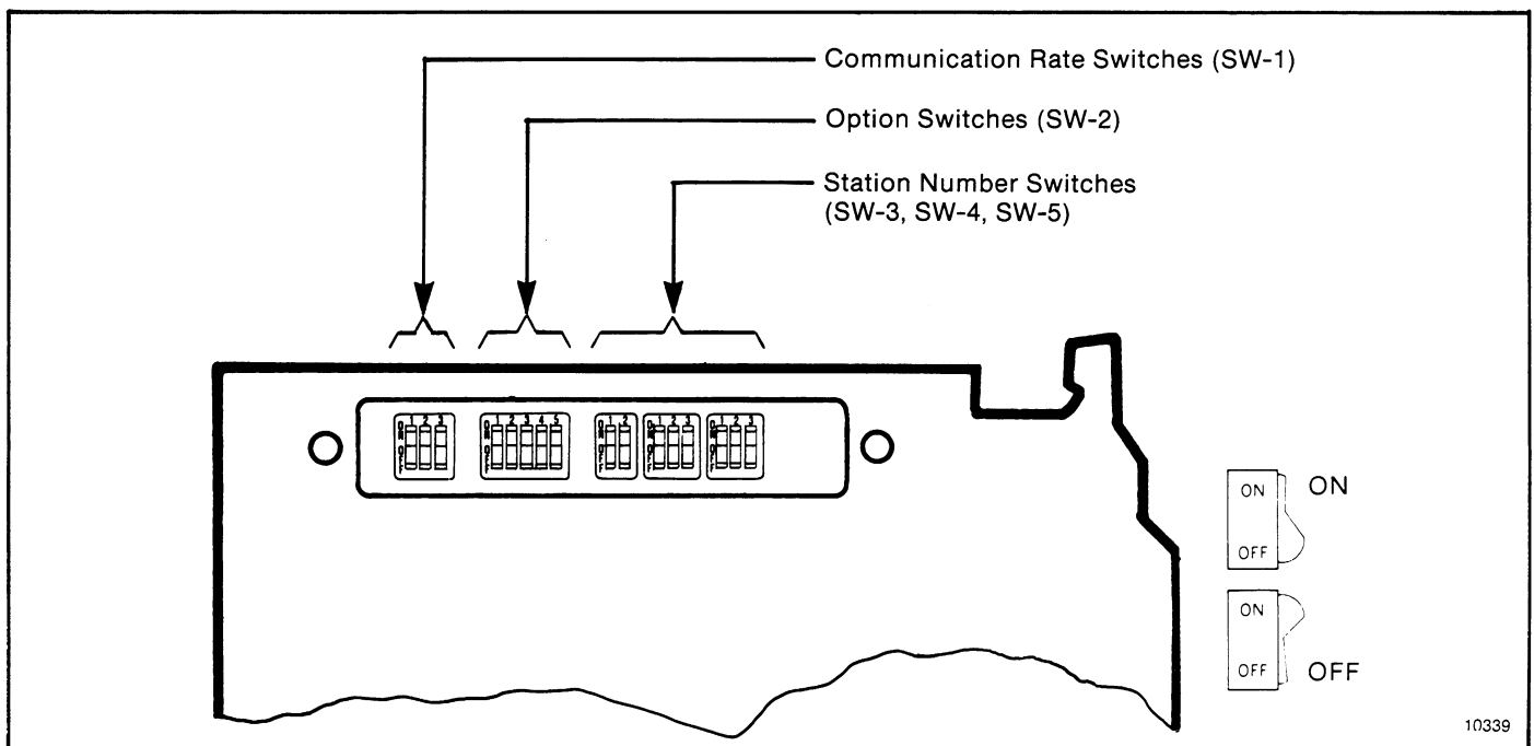
Figure 4.1 — Switch Assembly Locations
