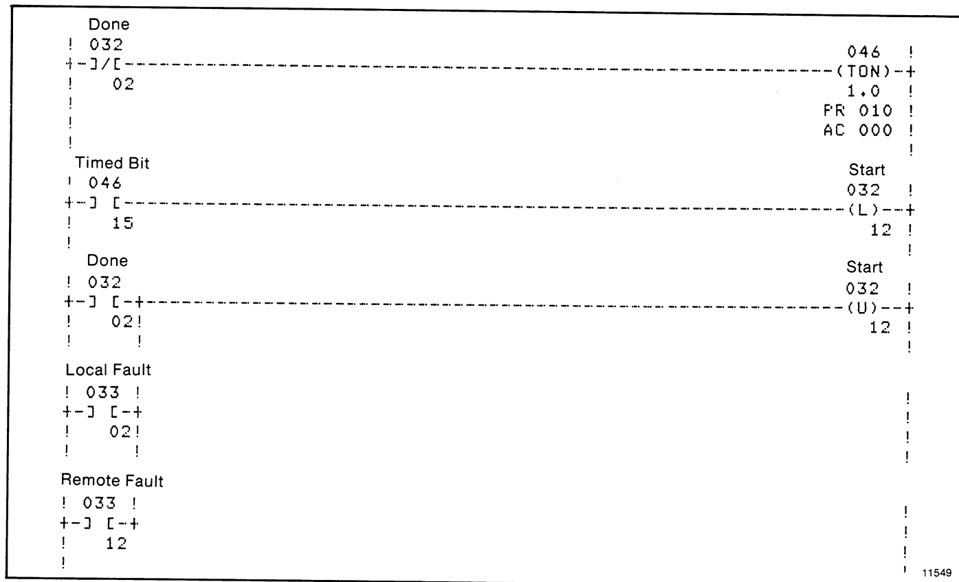
Figure 5.16 — Timer-Initiated Command
