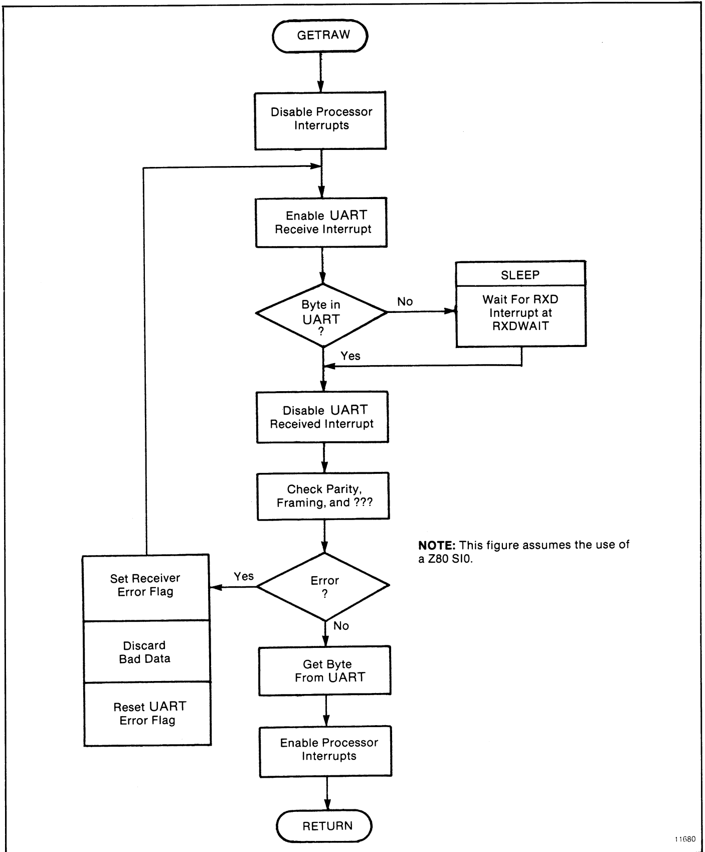
Figure D.28 — GETRAW Subroutine
