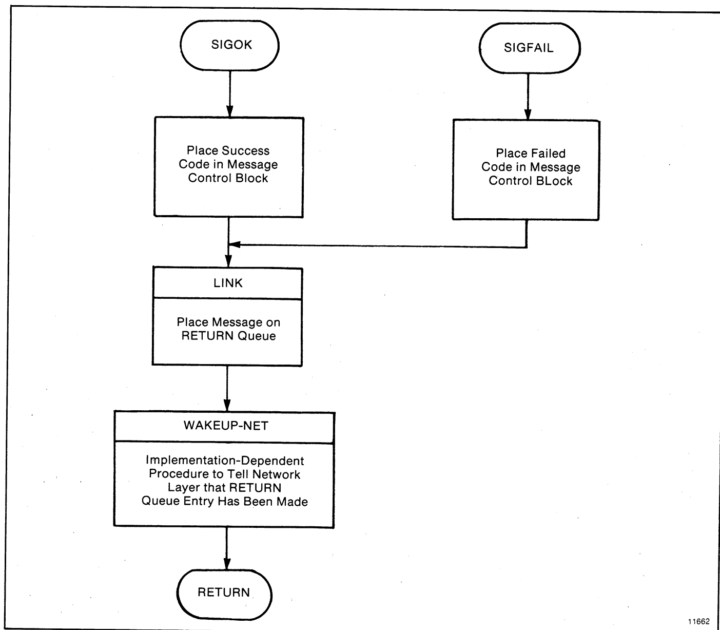
Figure D.10 — SIGOK/SIGFAIL Subroutine
