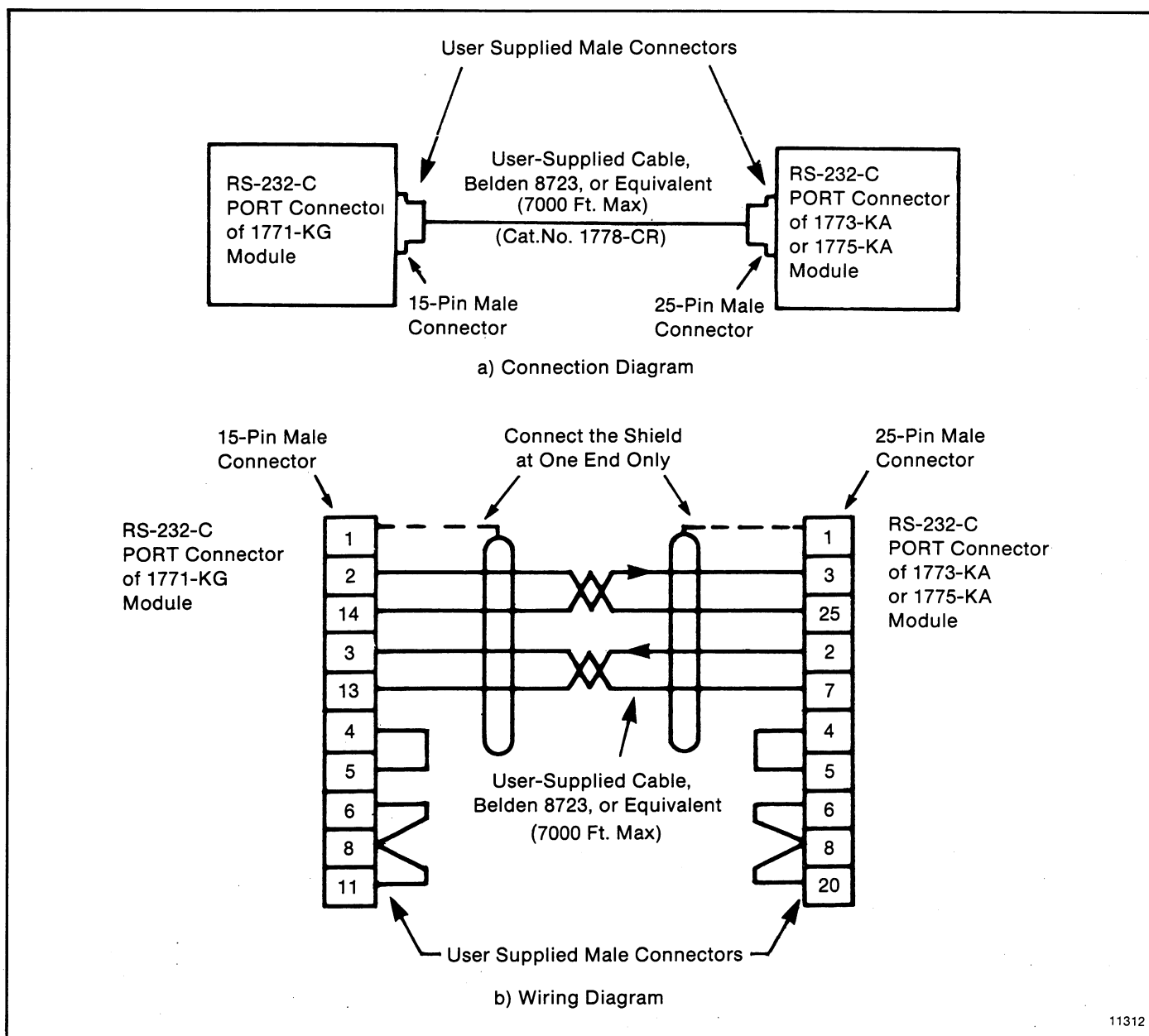
Figure 4.13 — Connection to 1773-KA or 1775-KA Module
