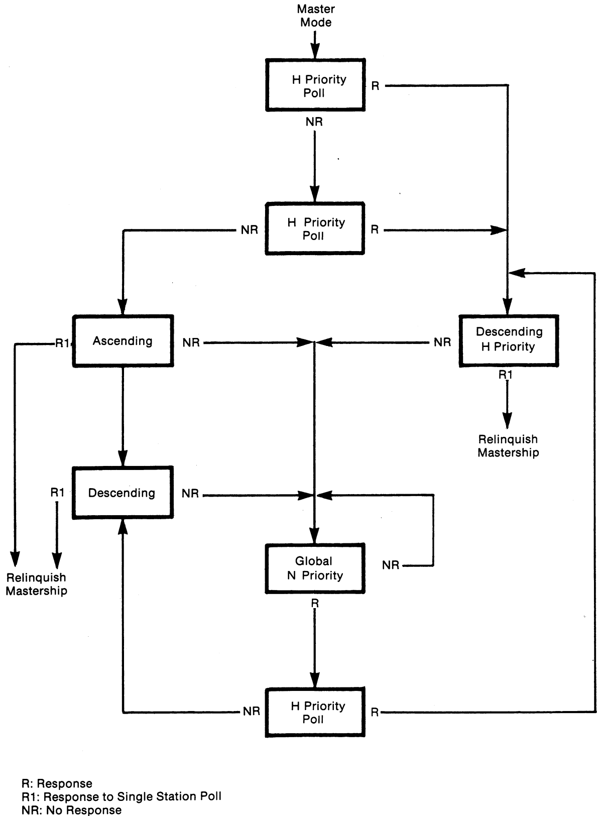
Figure 3.3 — Polling Process
