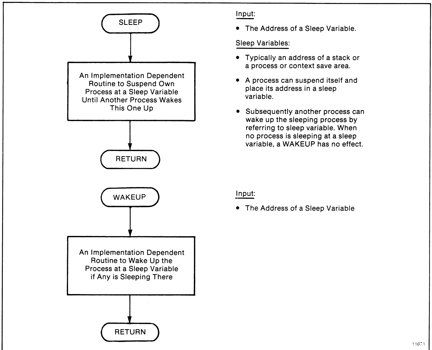
Figure D.19 — SLEEP and WAKEUP Subroutines
