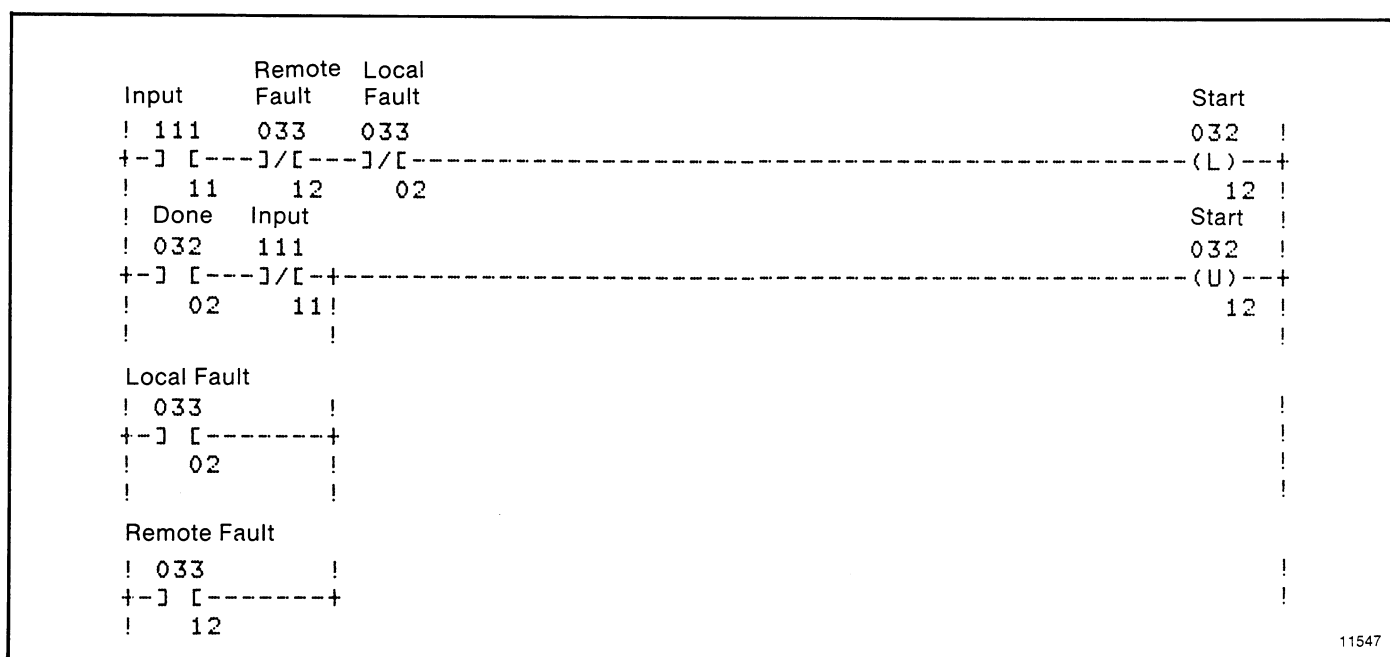
Figure 5.14 — Status-Initiated Command
