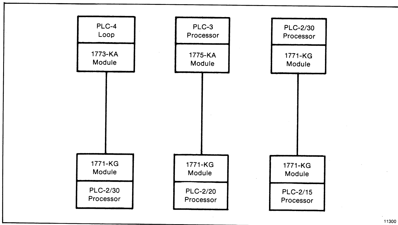
Figure 2.2 — Stand-Alone PC-to-PC Links
