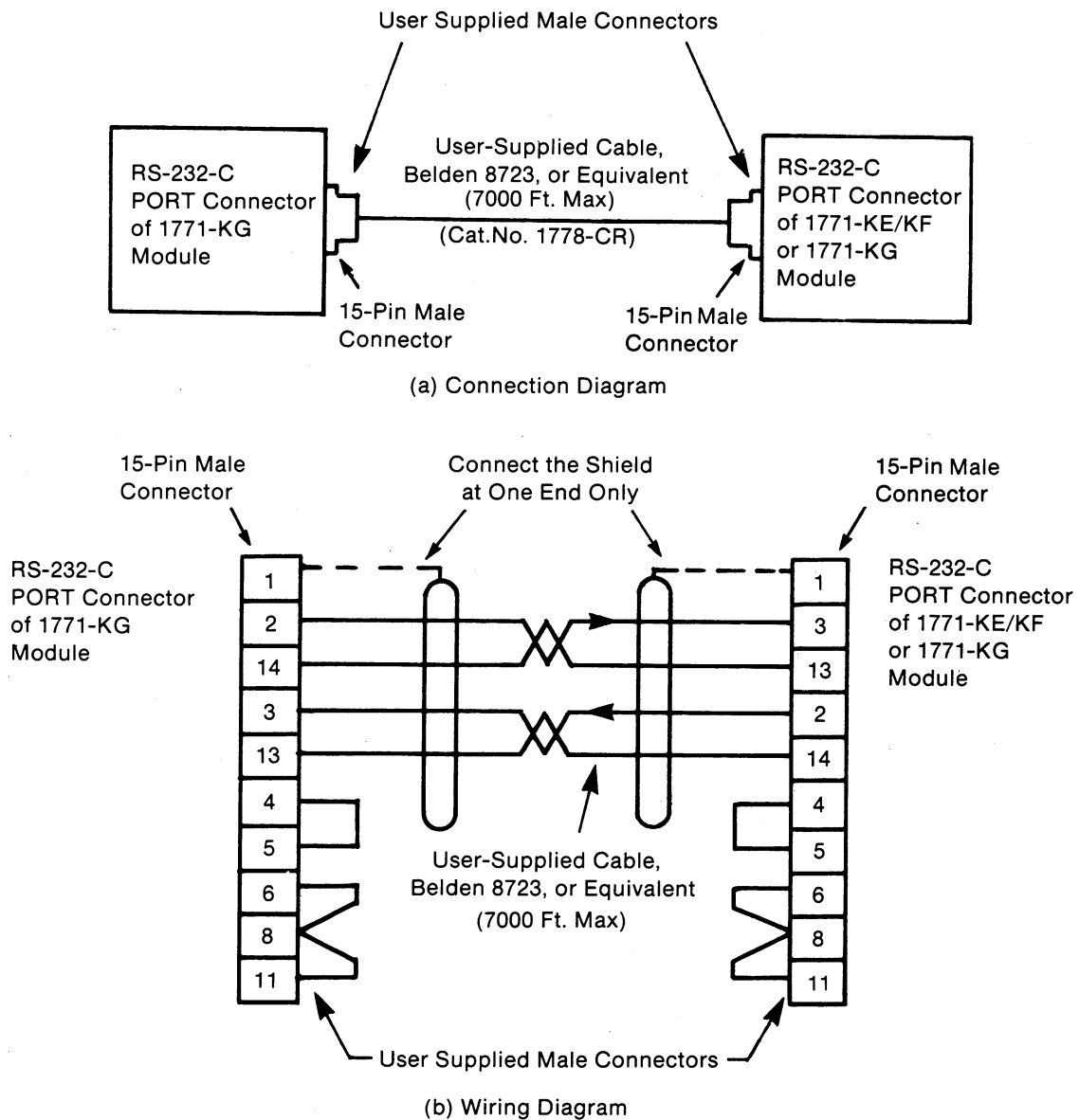
Figure 4.12 — Connection to 1771-KE/KF or Another 1771-KG Module
