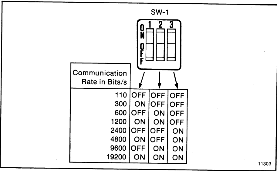
Figure 4.2 — Communication Rate Switch Settings
