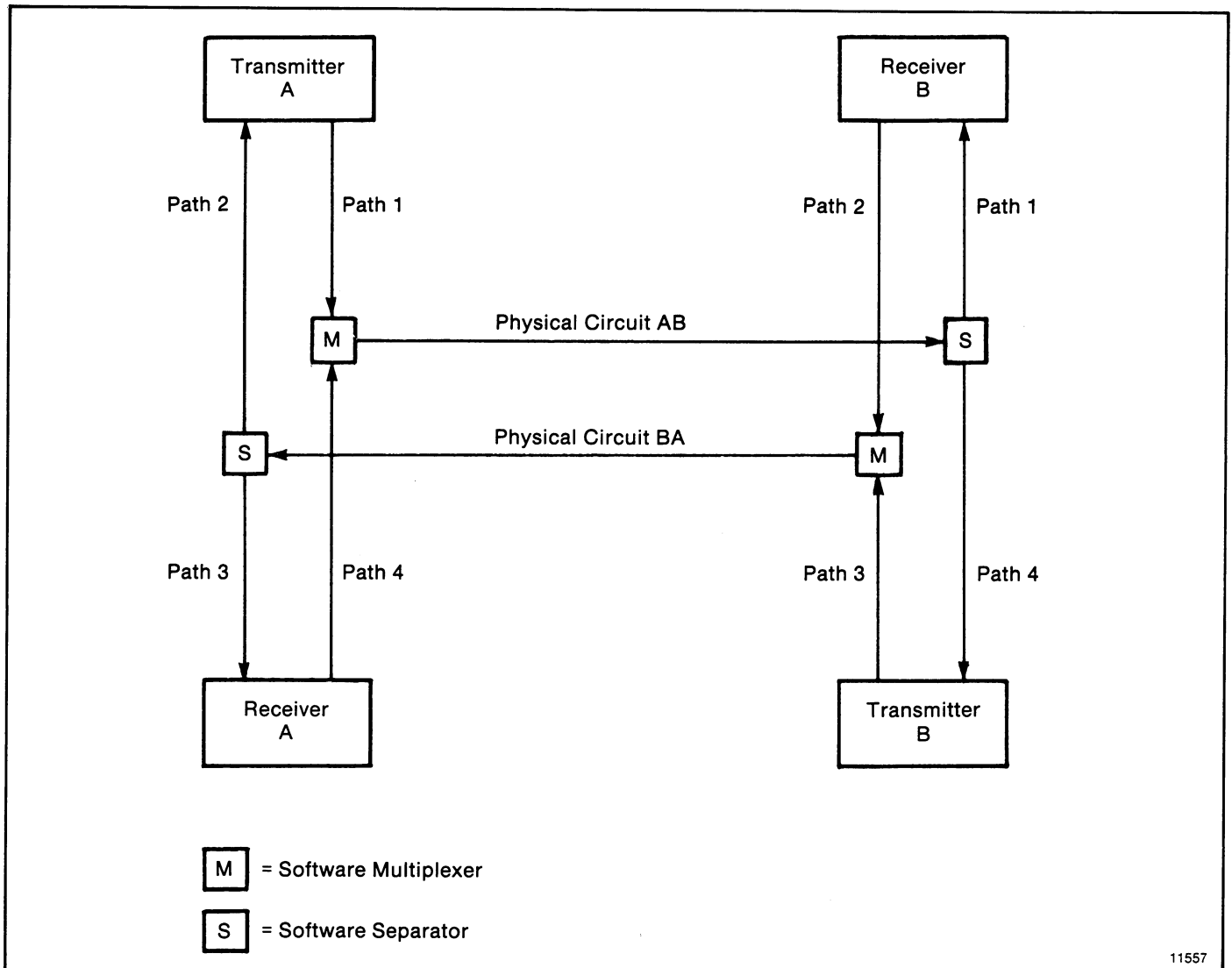
Figure 6.3 — Software Implementation of Data Paths
