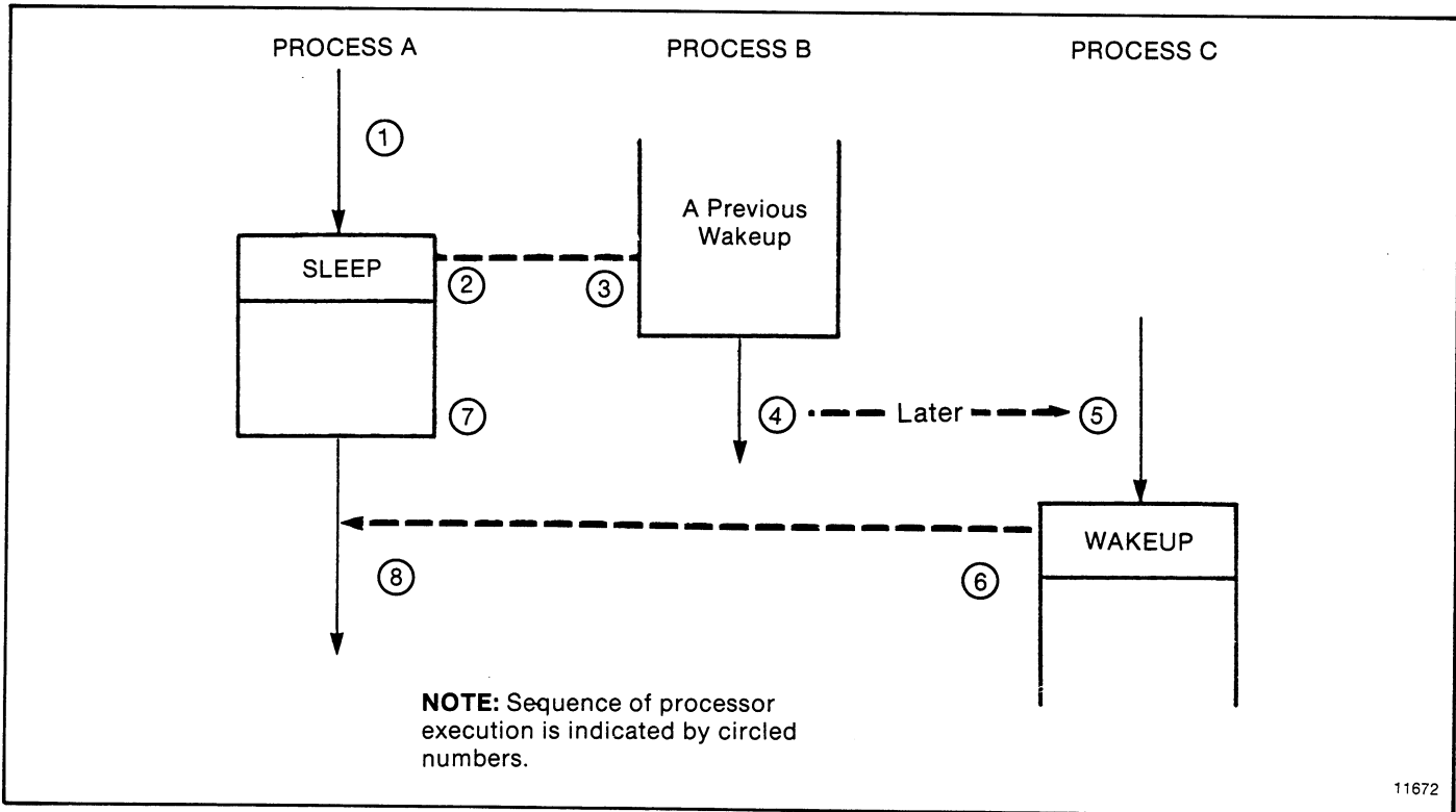
Figure D.20 — SLEEP and WAKEUP Interaction
