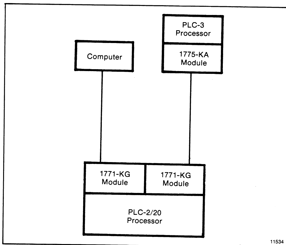
Figure 2.5 — A Second RS-232-C Link for PLC-2-Family Processor
