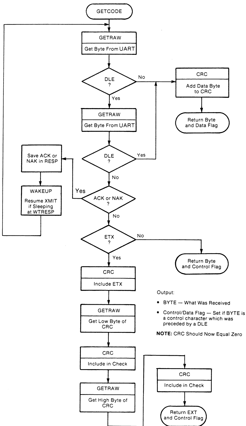
Figure D.27 — GETCODE Subroutine
