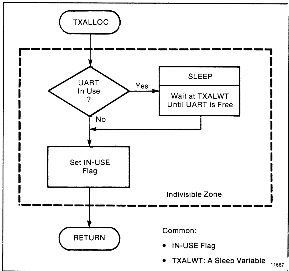
Figure D.15 — TXALLOC Subroutine
