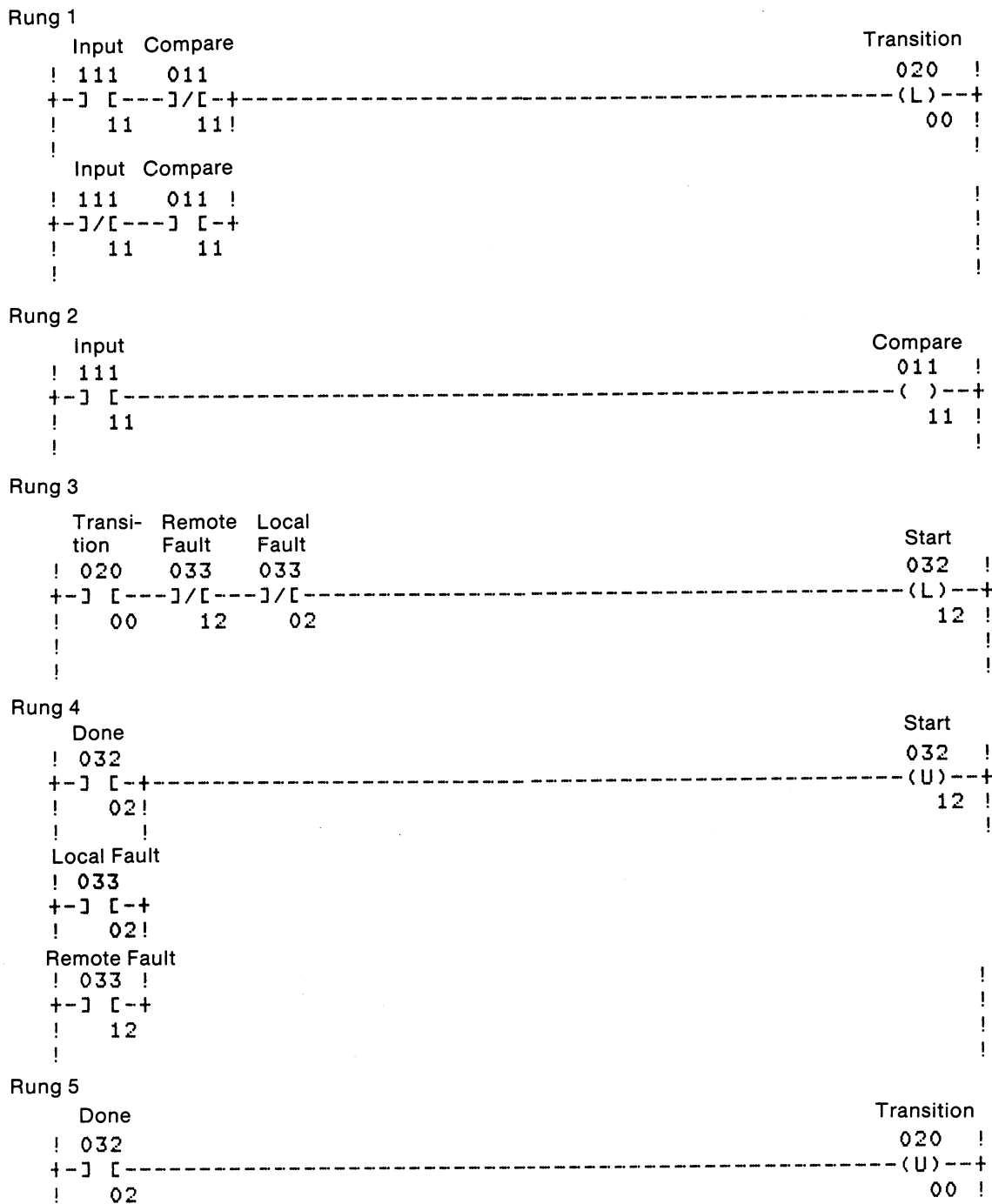
Figure 5.15 — Transition-Initiated Command
