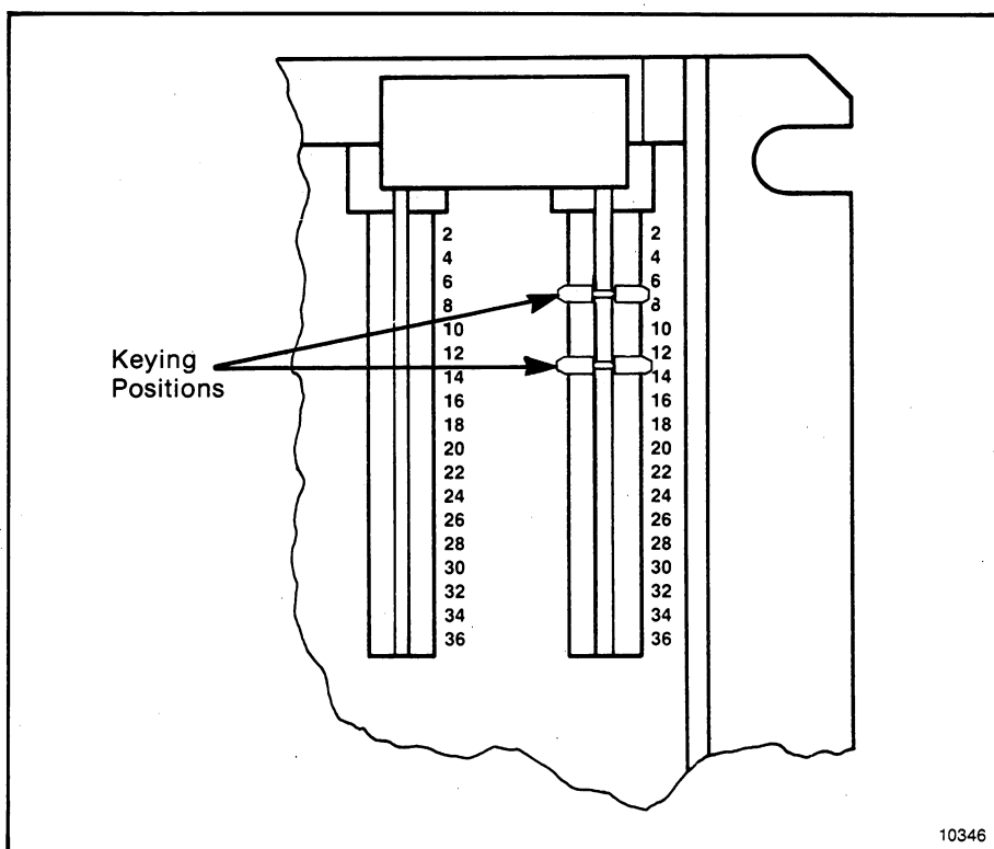
Figure 4.5 — Keying Diagram
