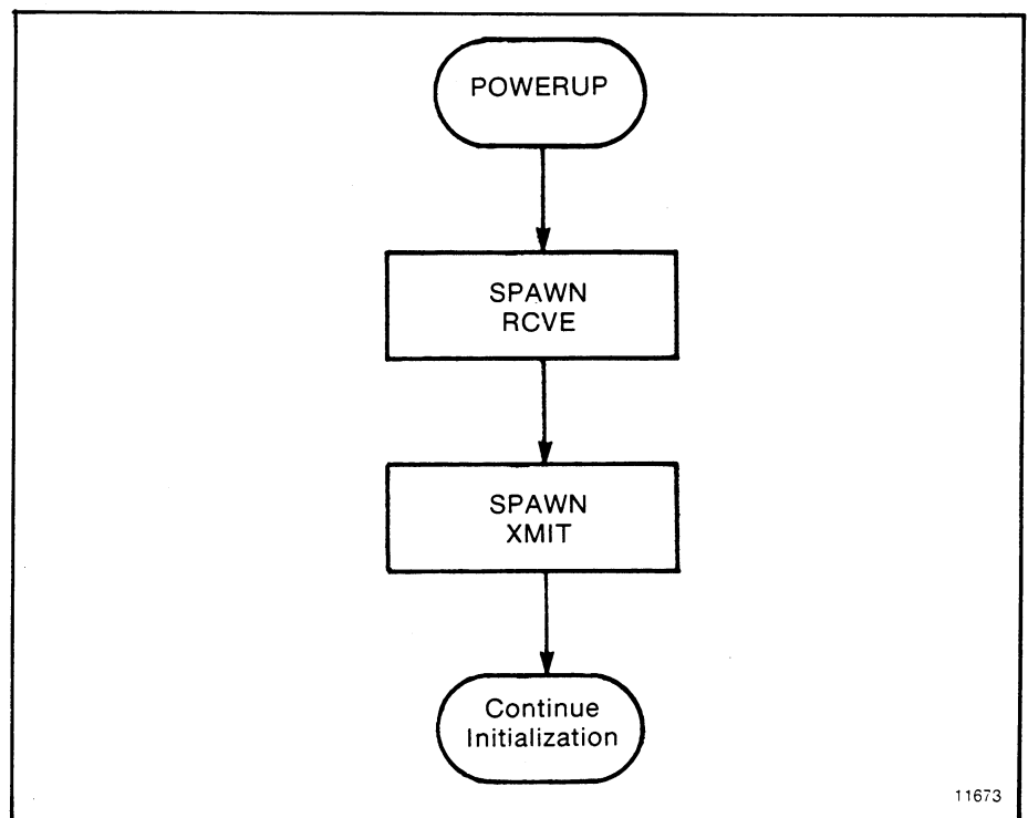
Figure D.21 — POWERUP Subroutine
