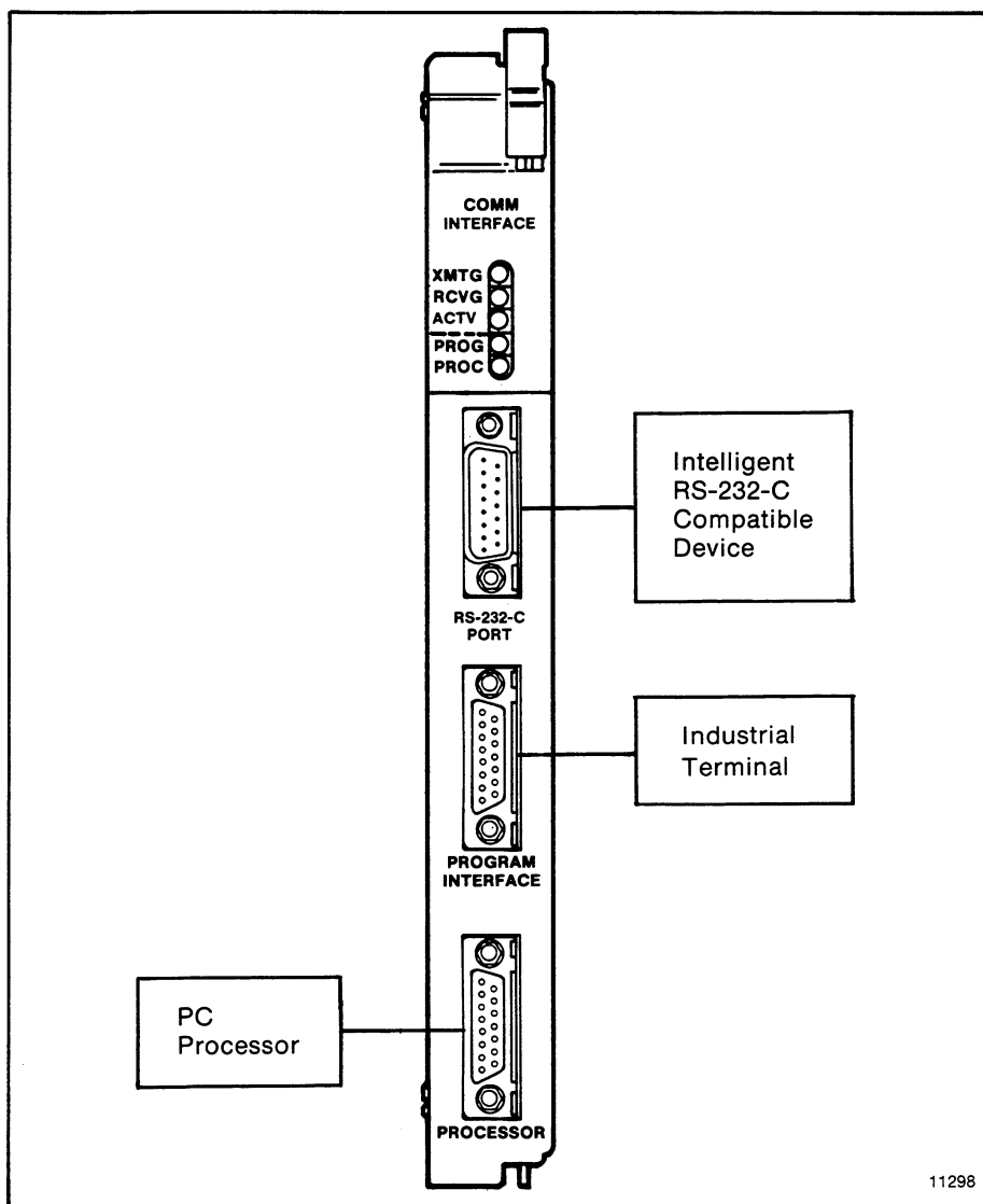
Figure 1.2 — Communication Connections
