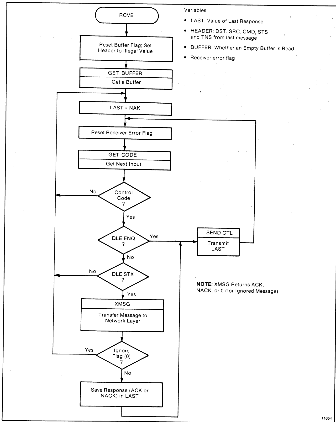
Figure D.3 — Receiver Routine for Full-Duplex Protocol
