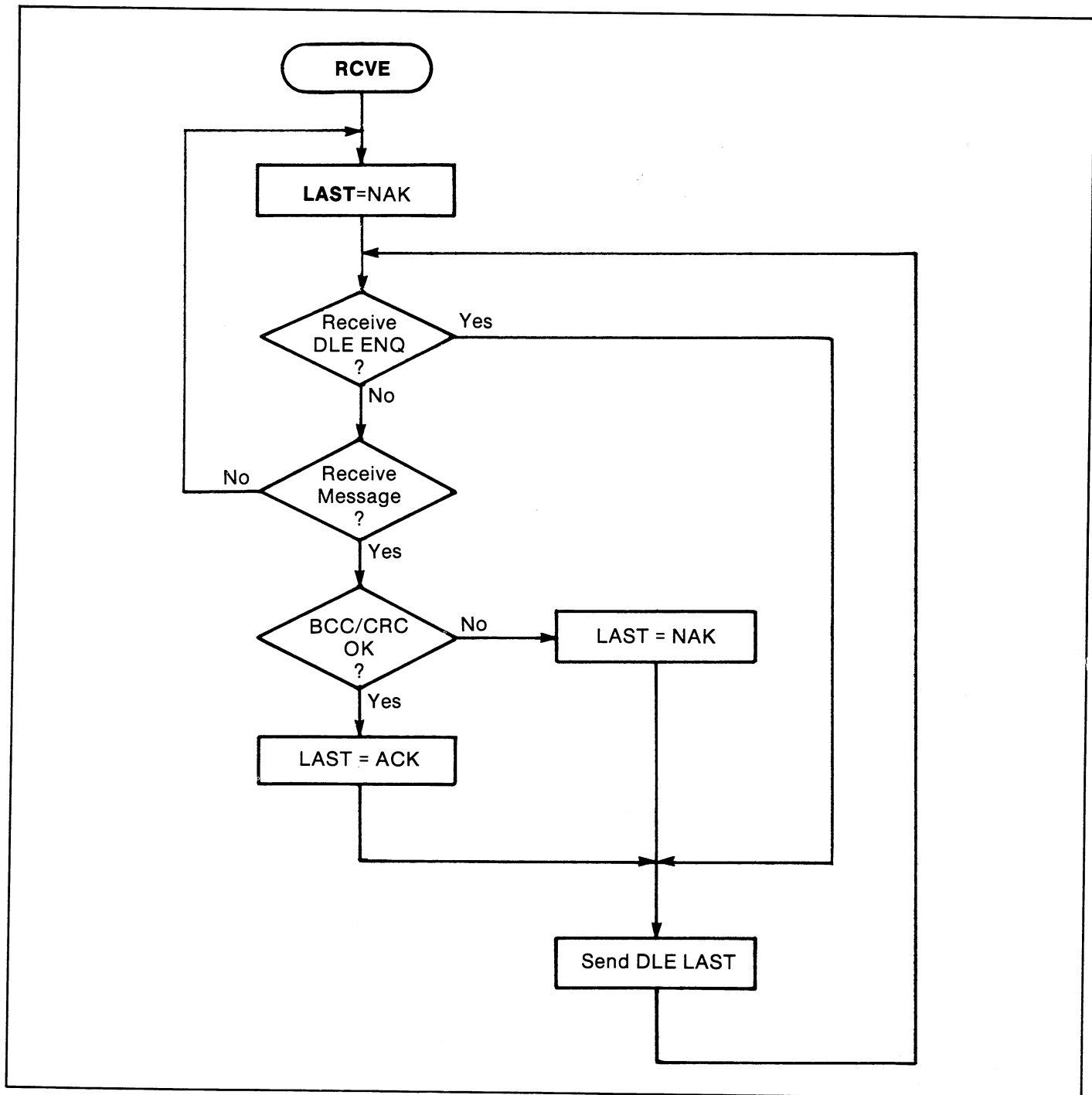
Figure 6.8 — Receiver for Full-Duplex Protocol
