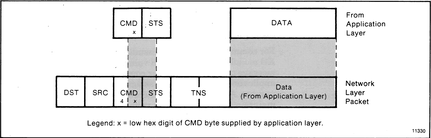
Figure 6.27 — Reply Message Packet Format
