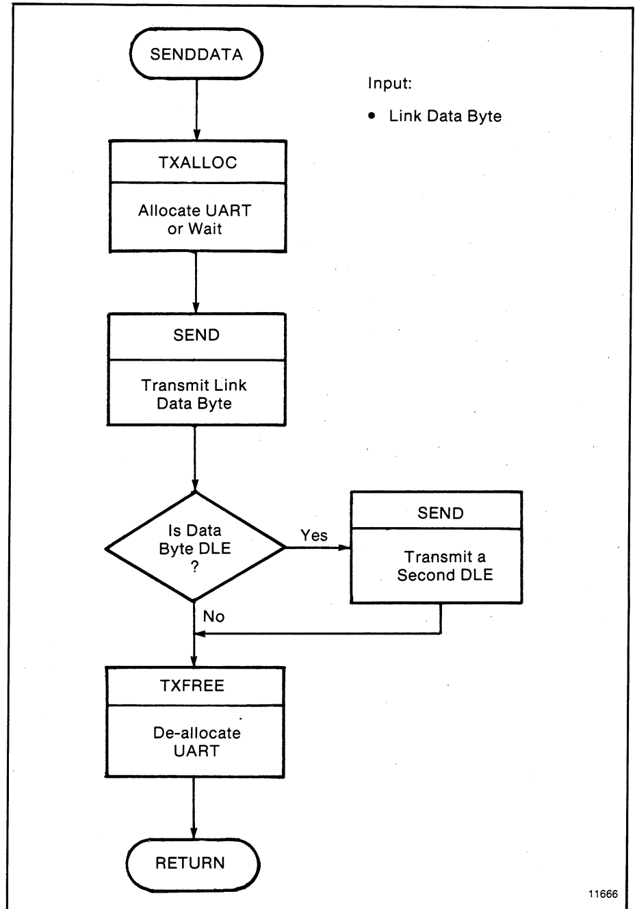
Figure D.14 — SENDDATA Subroutine
