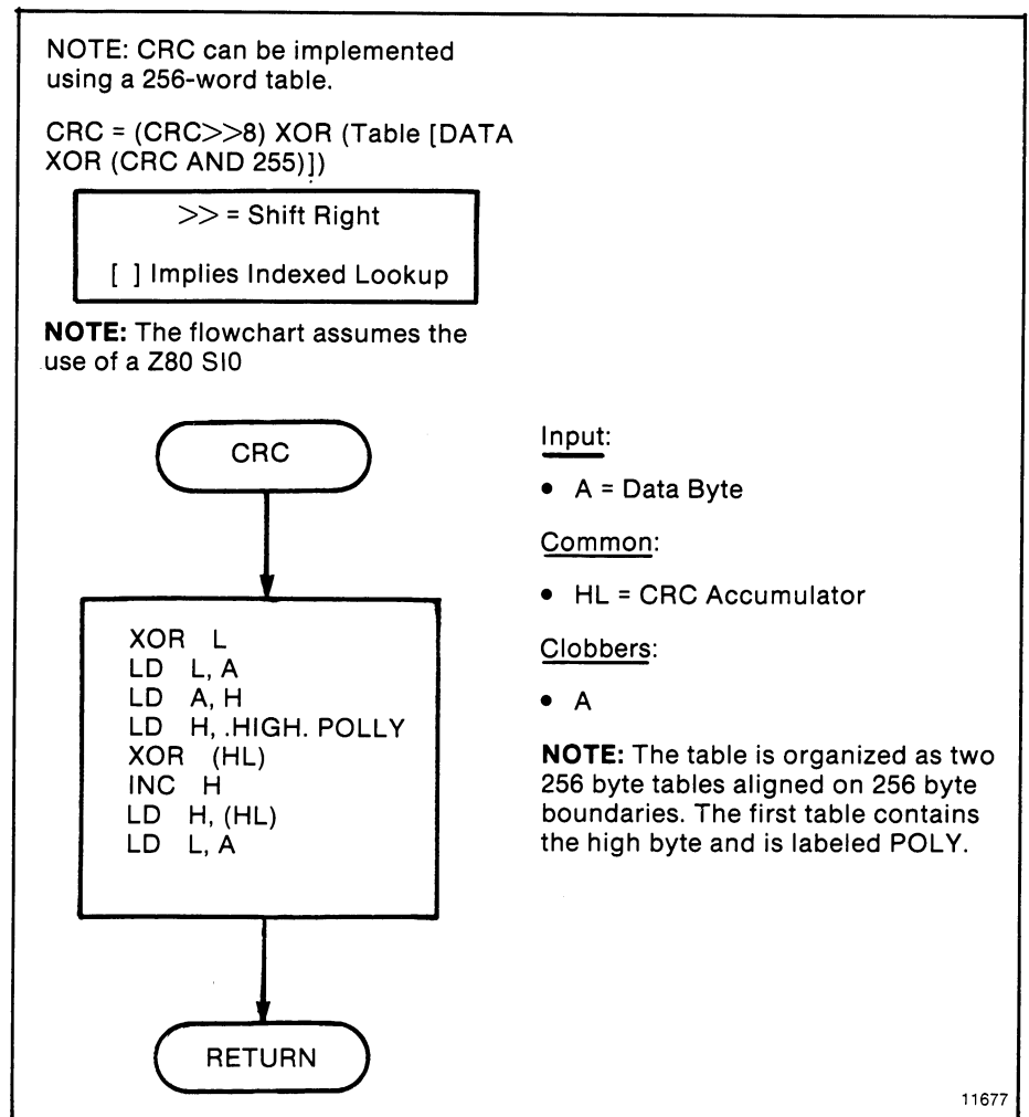
Figure D.25 — CRC Subroutine
