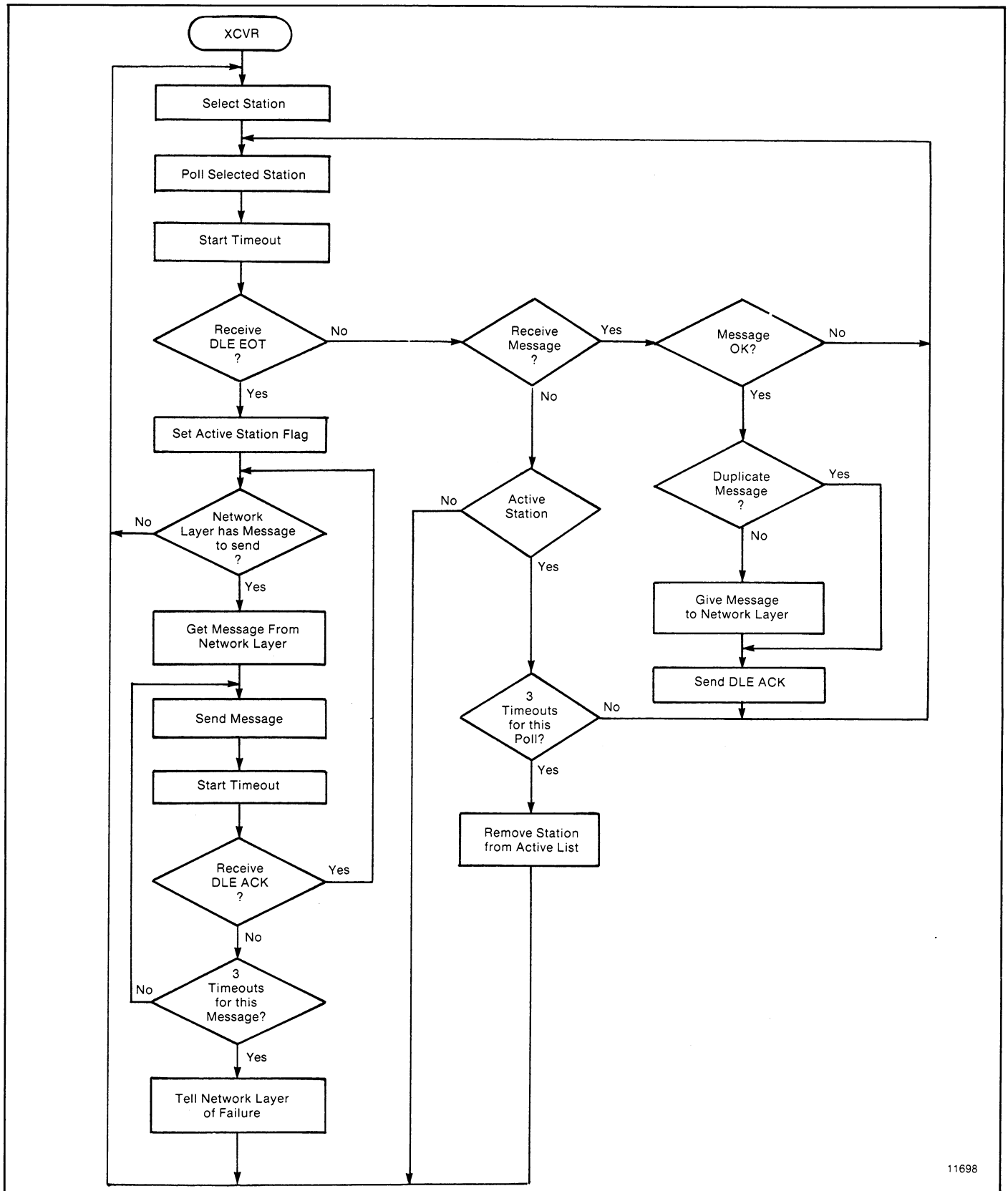
Figure 6.16 — Implementation of Half-Duplex Protocol
