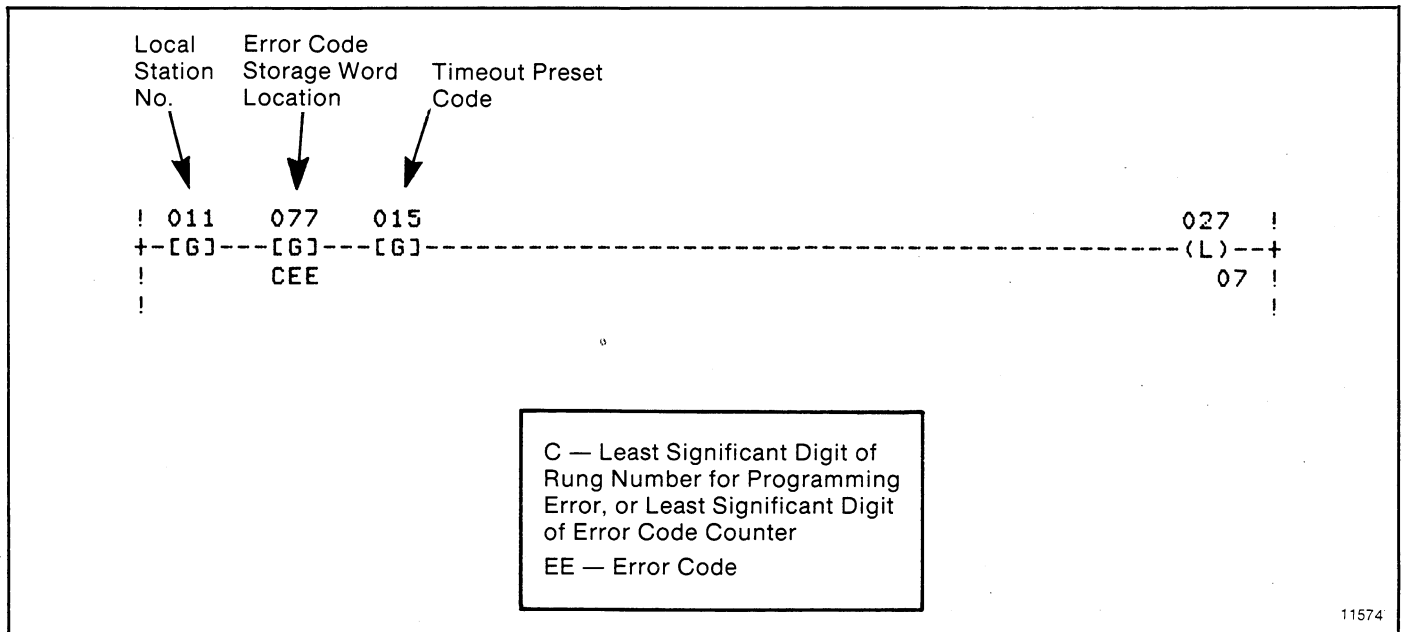
Figure 7.3 — Header Rung
