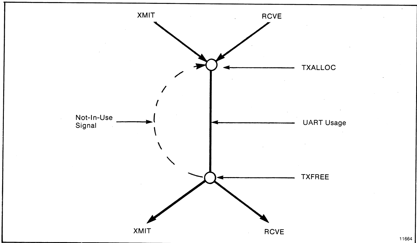
Figure D.11 — Sharing the Transmit Side of the UART
