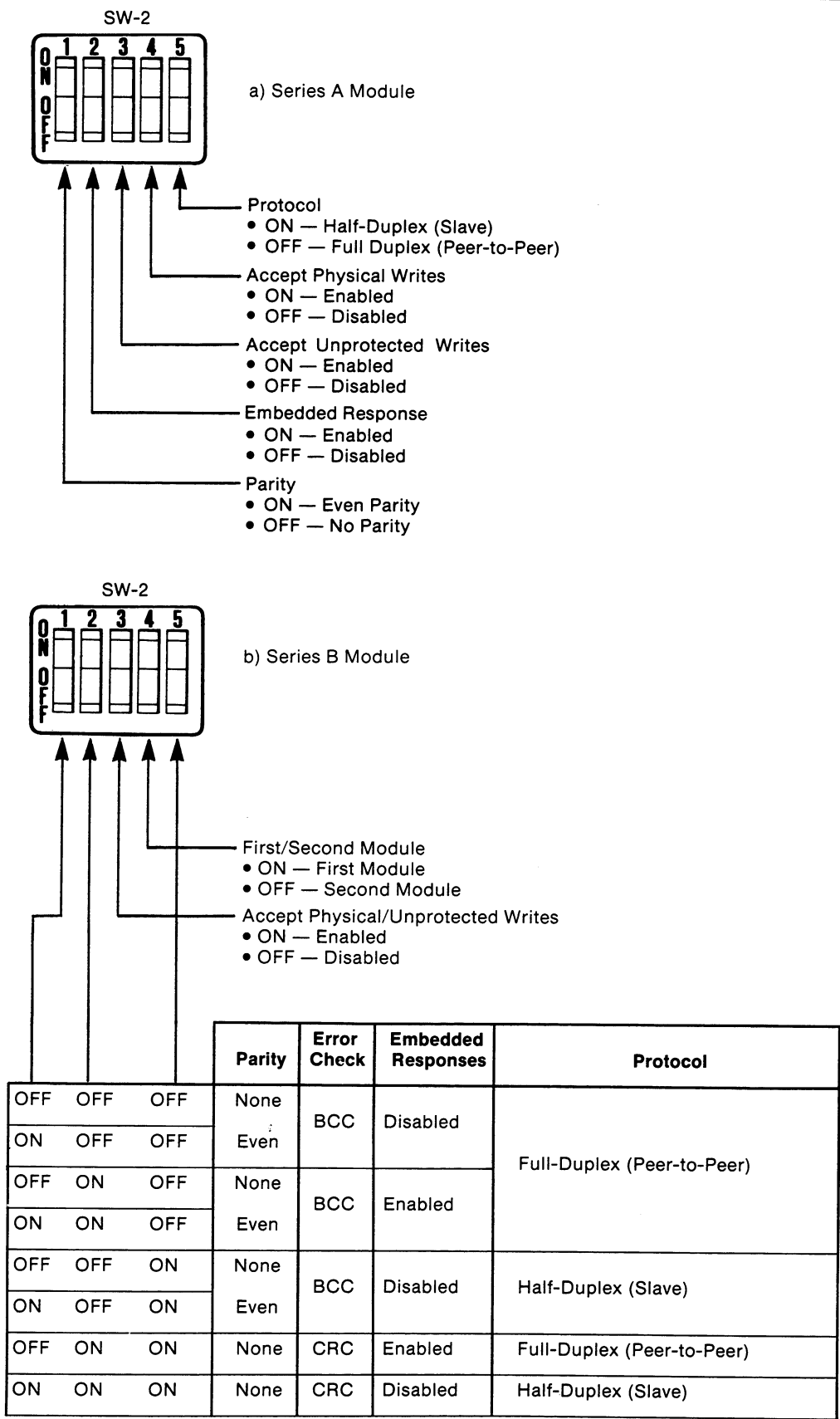
Figure 4.3 — Option Switch Settings
