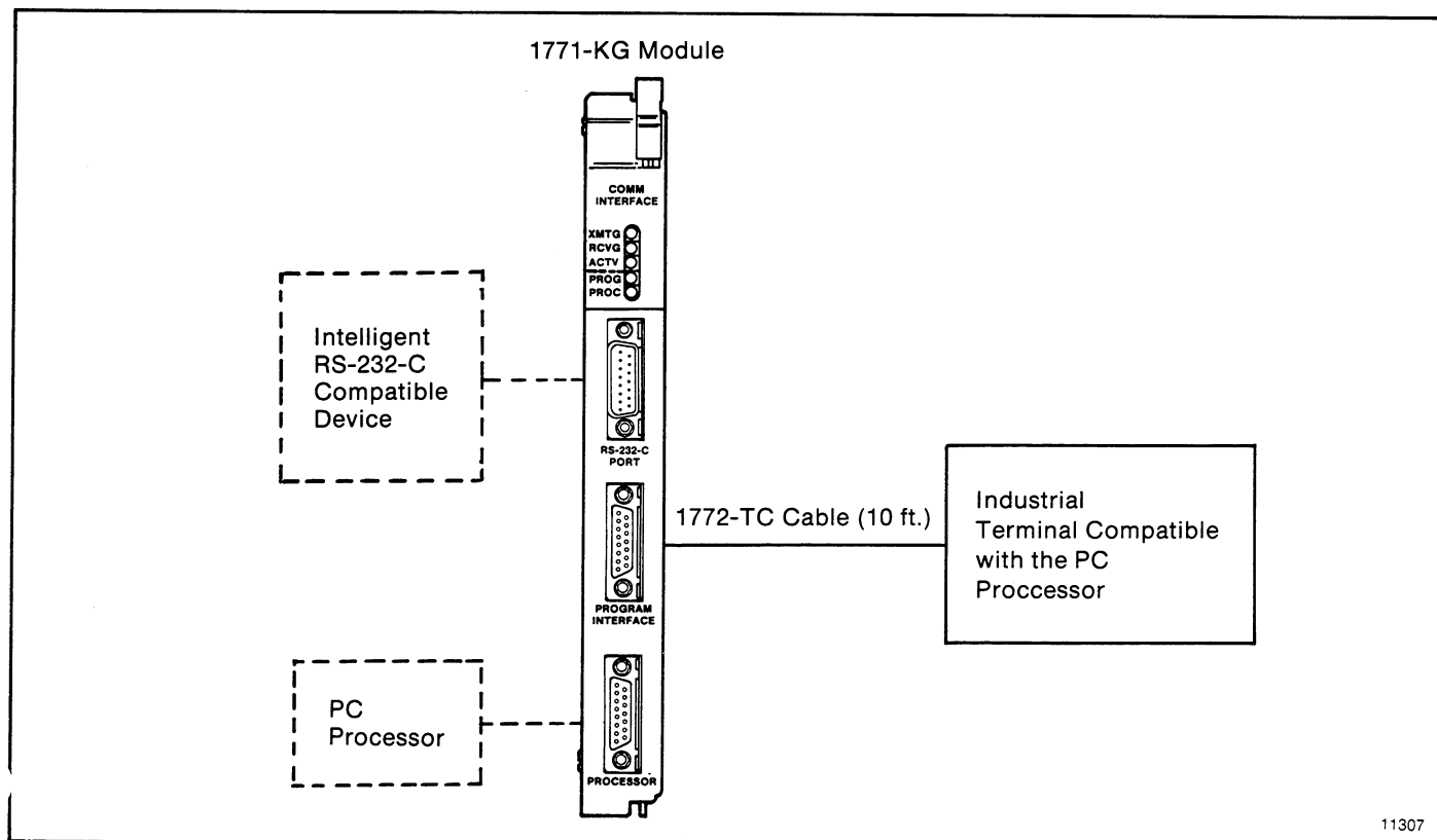
Figure 4.7 — Connection to a Programming Terminal
