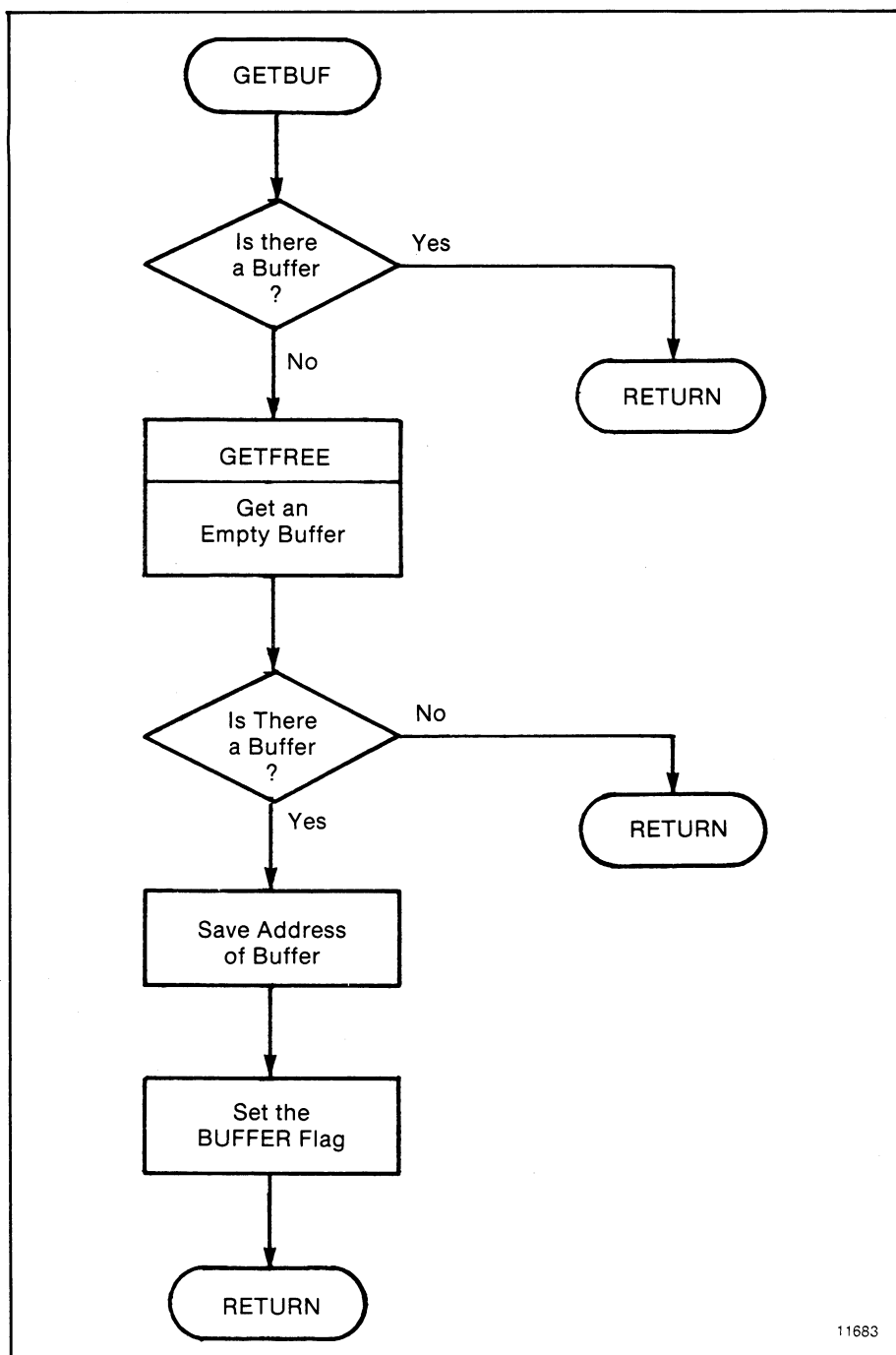
Figure D.31 — GETBUF Subroutine
