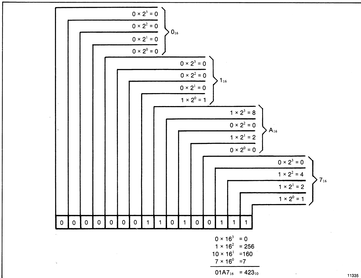
Figure C.4 — Hexadecimal Numbers
