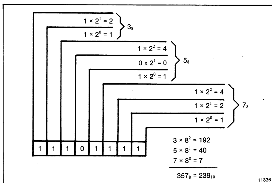
Figure C.5 — Octal Numbers
