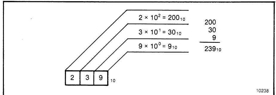
Figure C.3 — Decimal Numbers
