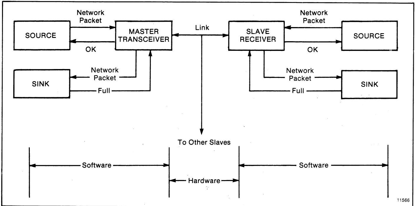
Figure 6.15 — Slave Transceiver
