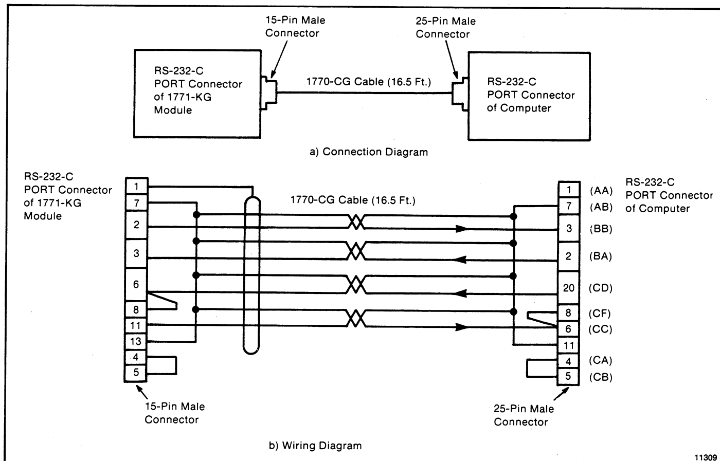
Figure 4.10 — Connection to a Computer
