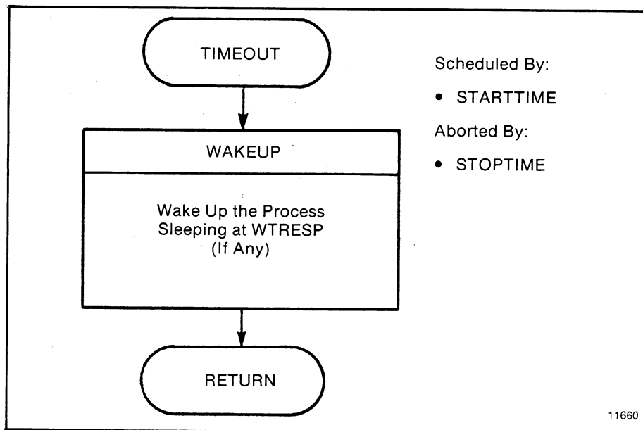
Figure D.8 — TIMEOUT Subroutine
