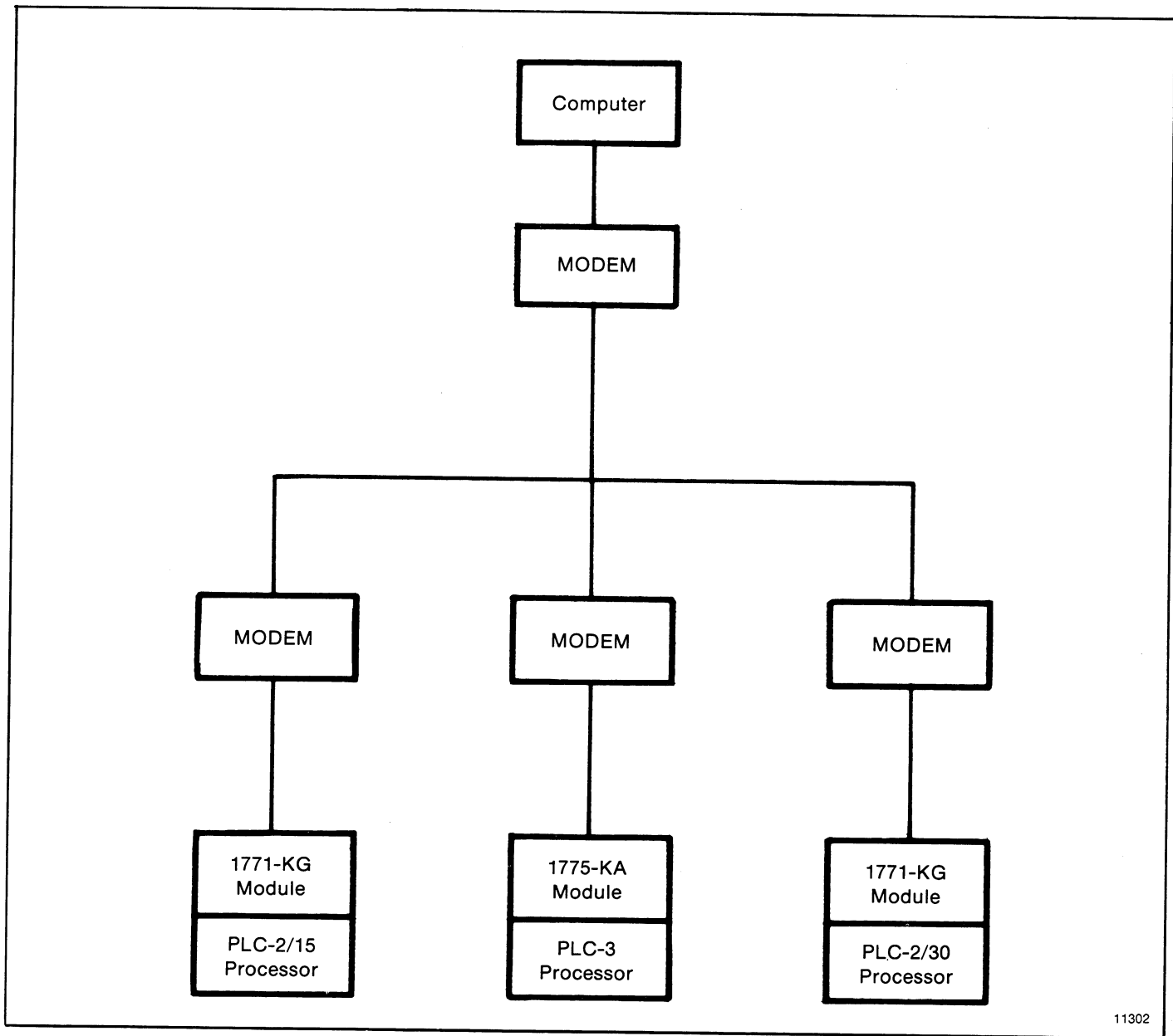
Figure 2.4 — Stand-Alone Multi-Drop Link to a Computer
