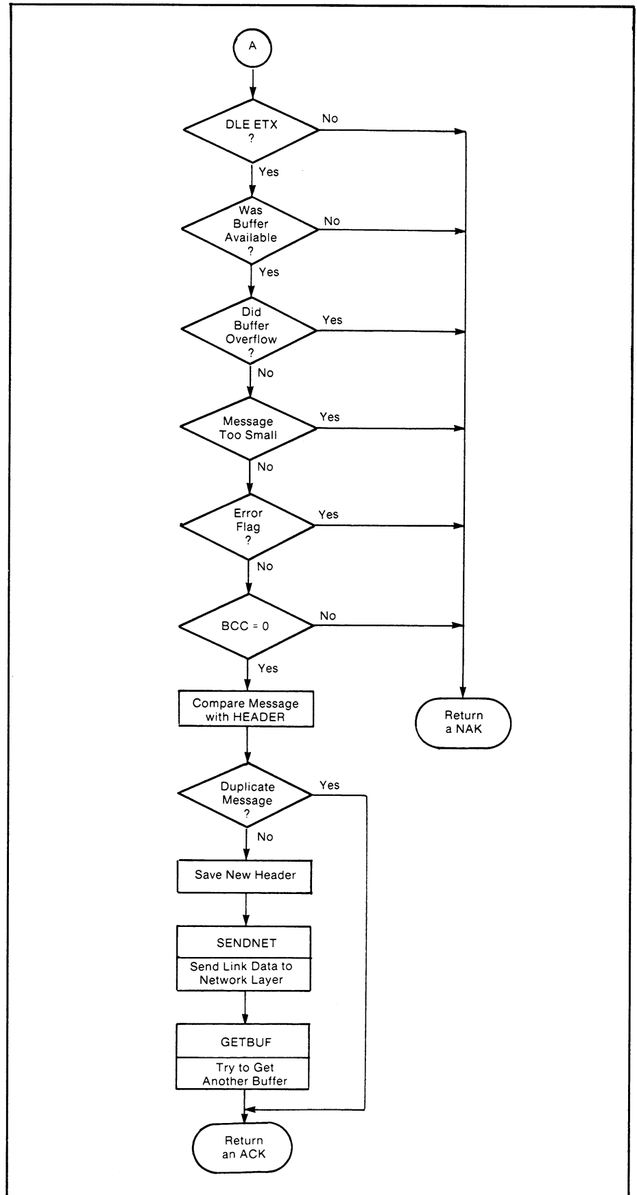
Figure D.26 — XMSG Subroutine (Continued)
