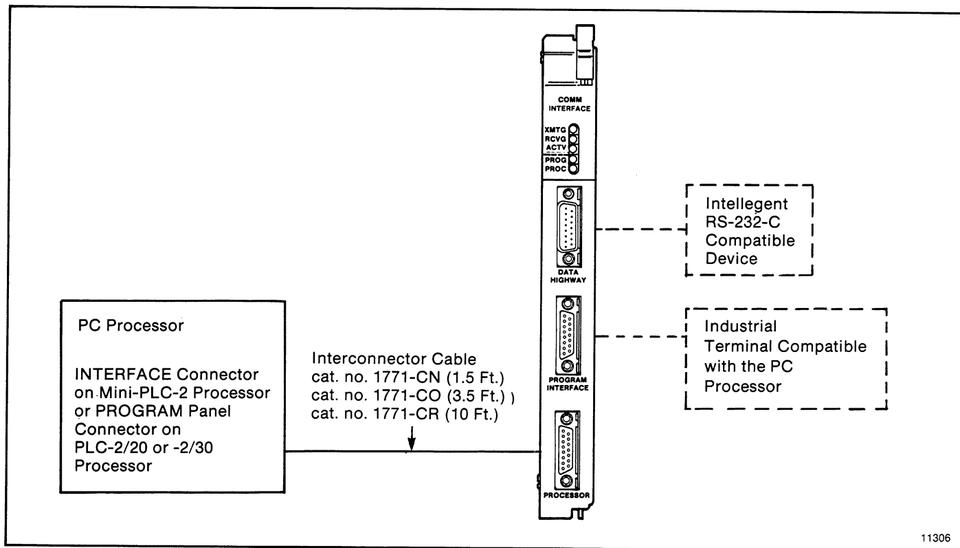
Figure 4.6 — Connection to the PC Processor
