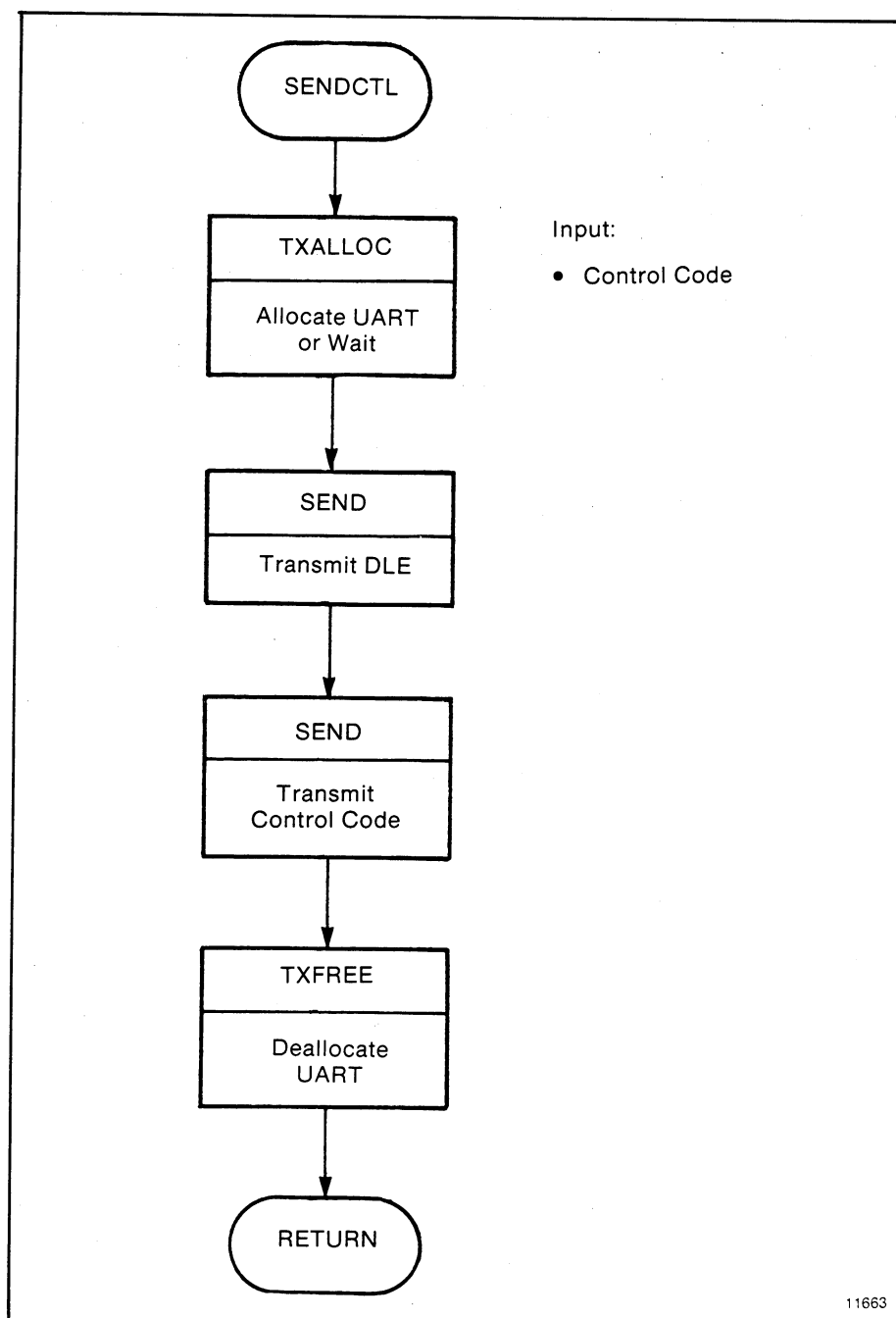
Figure D.12 — SENDCTL Subroutine
