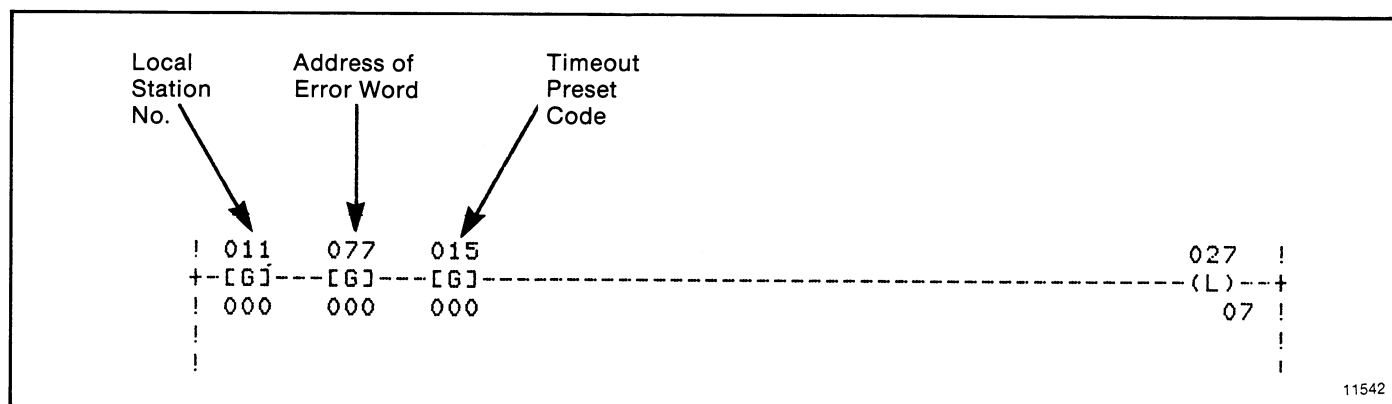
Figure 5.2 — Header Rung
