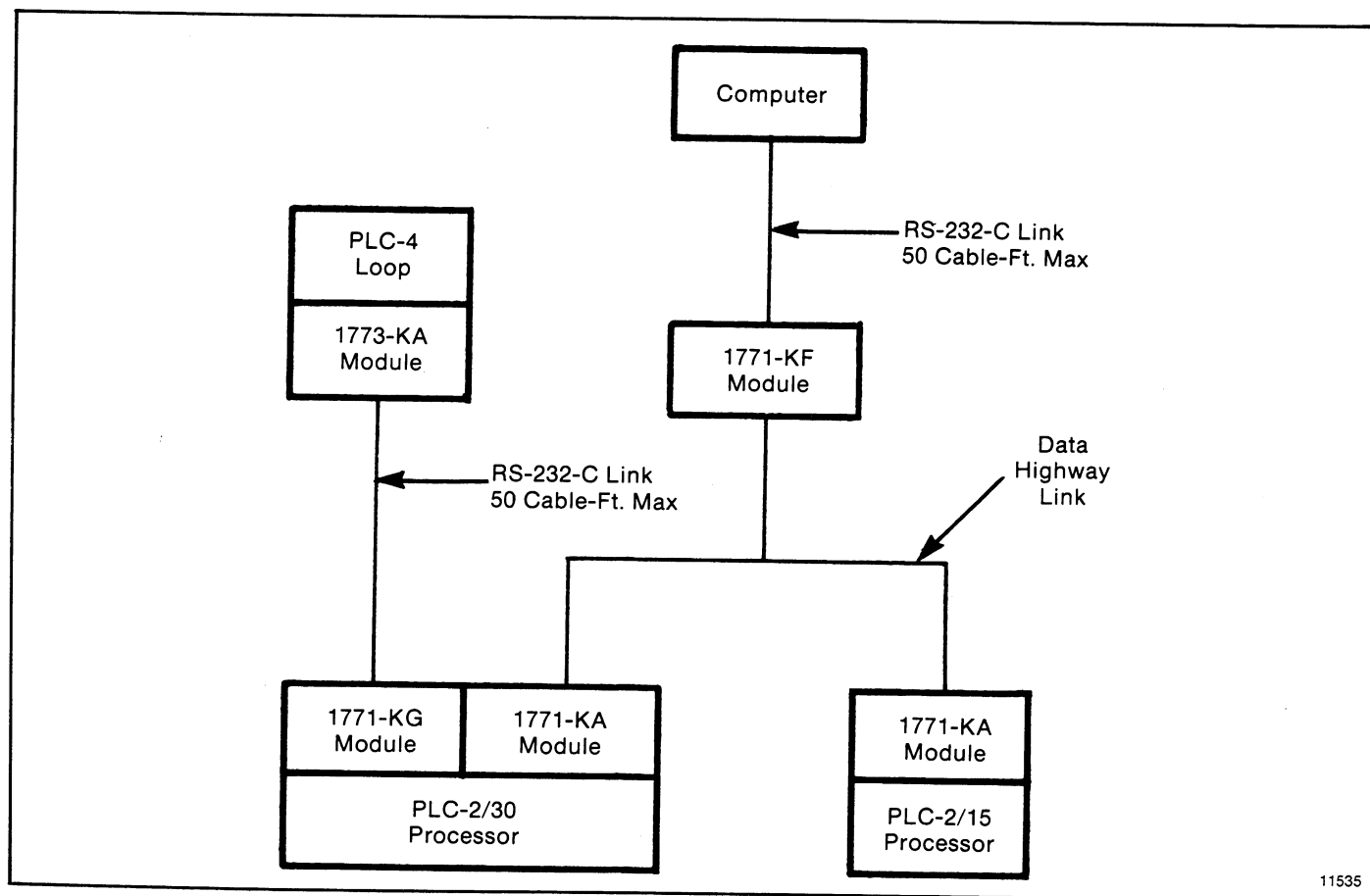
Figure 2.6 — An RS-232-C Link and a Data Highway Link for a PLC-2-Family Processor
