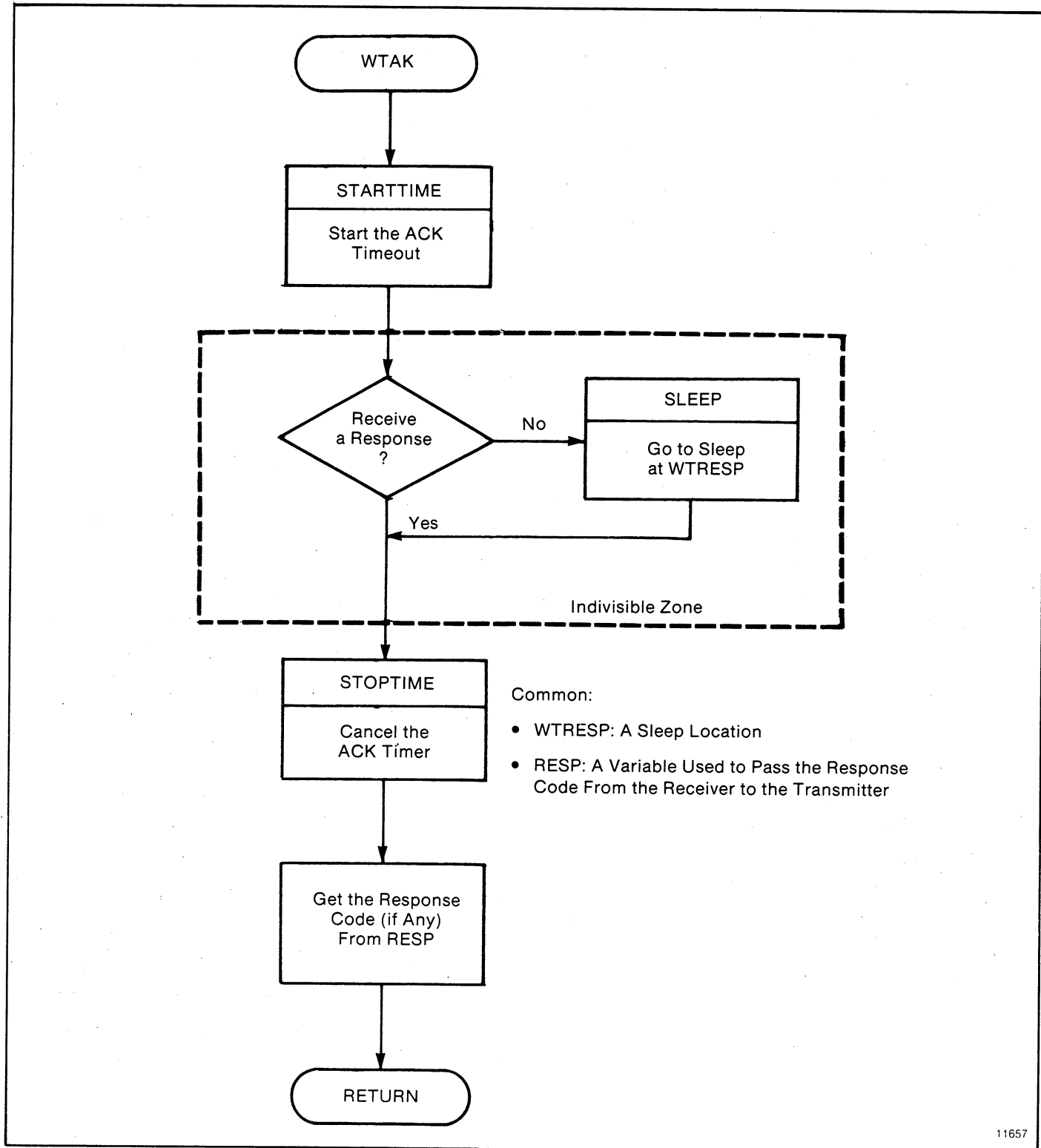
Figure D.5 — WTAK Subroutine
