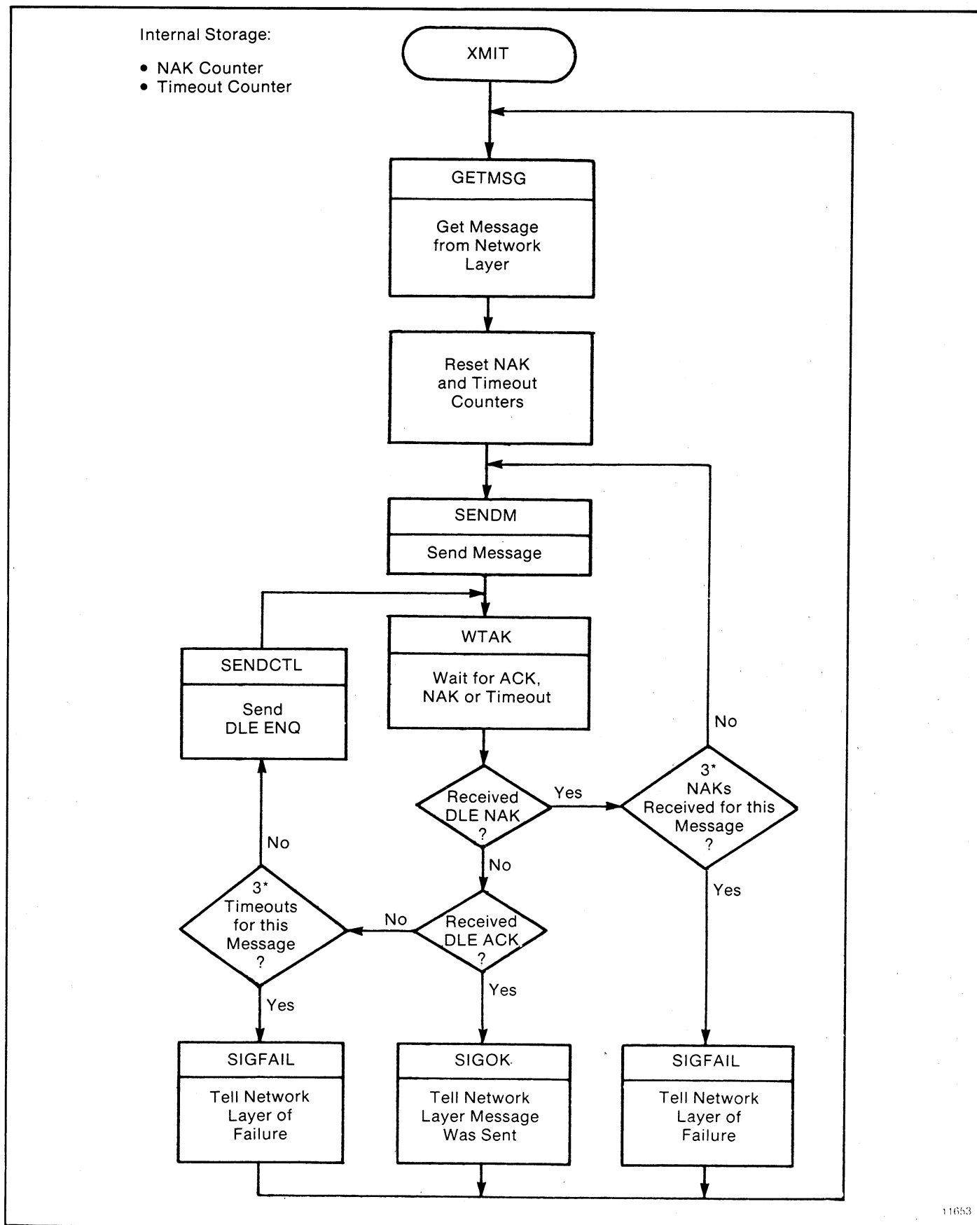
Figure D.2 — Transmitter Routine for Full Duplex Protocol
