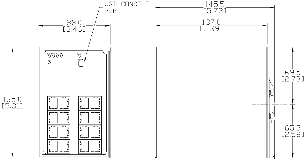
SE2-SW16M
