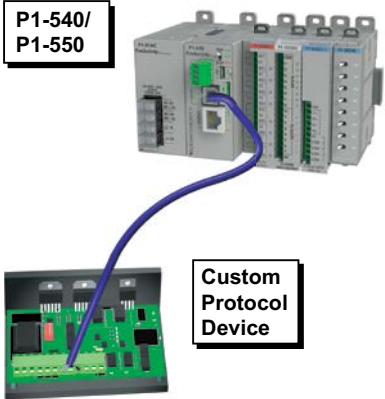
RS-232 Custom Protocol In and Out
