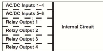
--- Basic Insulation _____ Reinforced Insulation P1-Mxxx 12DRS
