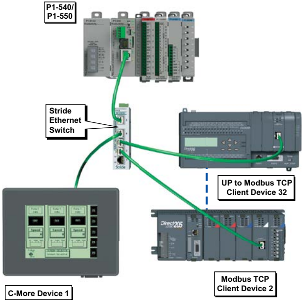
Modbus TCP Client (RX-WX)
