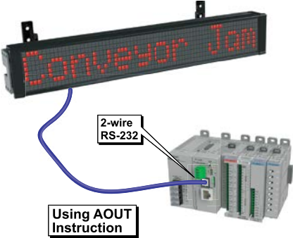
RS-232 ASCII Out Communication
