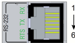
6-Pin RJ12 Female Modular Connector
