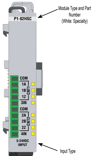
High-Speed Input Modules
