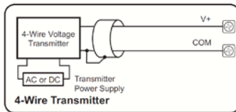
Voltage Input Circuits
