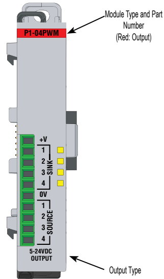
Pulse Width Modulation
