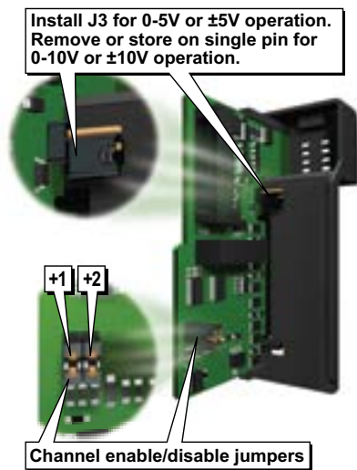
Jumper Location on Modules Having Date Code 0709G and Above (Single Circuit Board Design)
