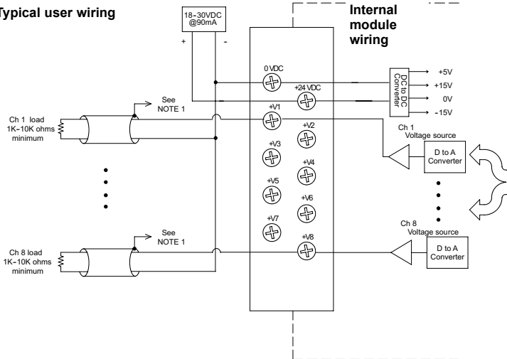
Typical user wiring
