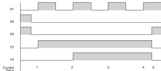
Counting Diagram
