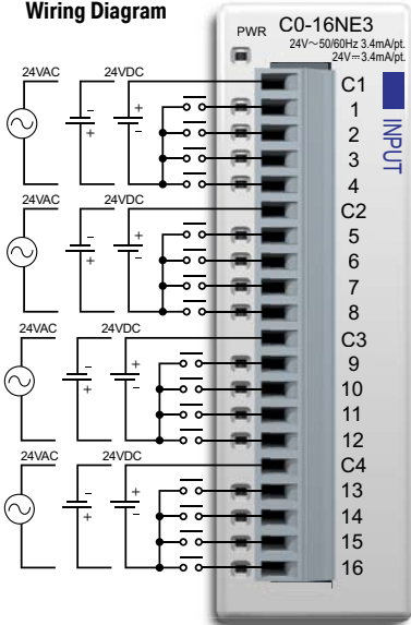
Wiring Diagram
