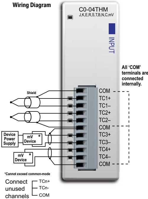
Wiring Diagram
