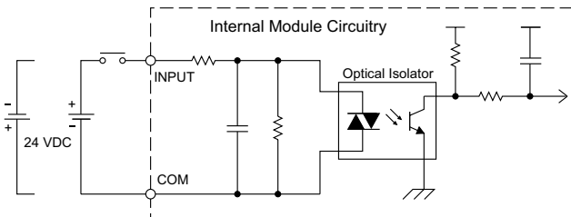
Equivalent Input Circuit
