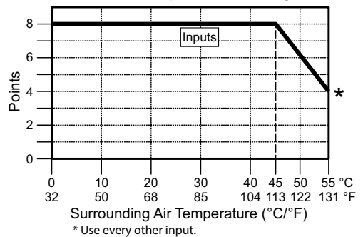
C0-10DRE-D Temperature Derating Chart
