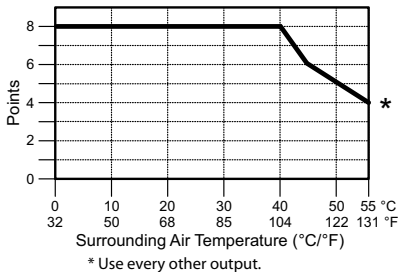
Output Temperature Derating Chart
