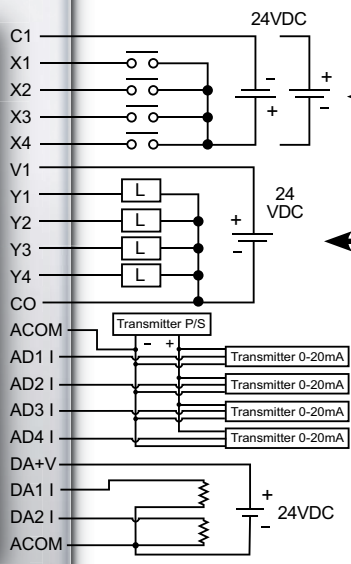
Wiring Diagram
