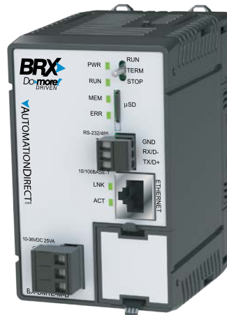
BX-DM1E-M-D 12–24 VDC
